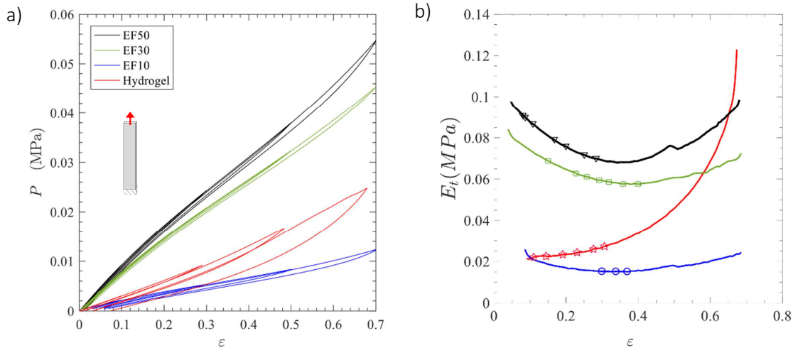
Figure 6.4: Tensile behaviour of the four polymers used for the vocal-fold replica during quasi-static and cyclic conditions : a) Piola-Kirchhoff stress P vs. Hencky strain \epsilon , b) Tangent modulus E_t as function of the applied strain \epsilon . For each material, symbols highlight the pre-strains \epsilon_{ap}^p which have been applied to the vocal-fold replica, and for which self-sustained oscillations could be observed.
