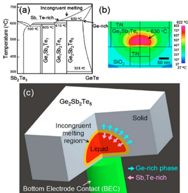
Fig. 2.13. a) The pseudobinary phase diagram between \text{Sb}_2\text{Te}_3 and \text{GeTe} for the analysis of the real PRAM device. b) The temperature profile simulation during the RESET operation. c) The phase separation model during the RESET operation. [112].
