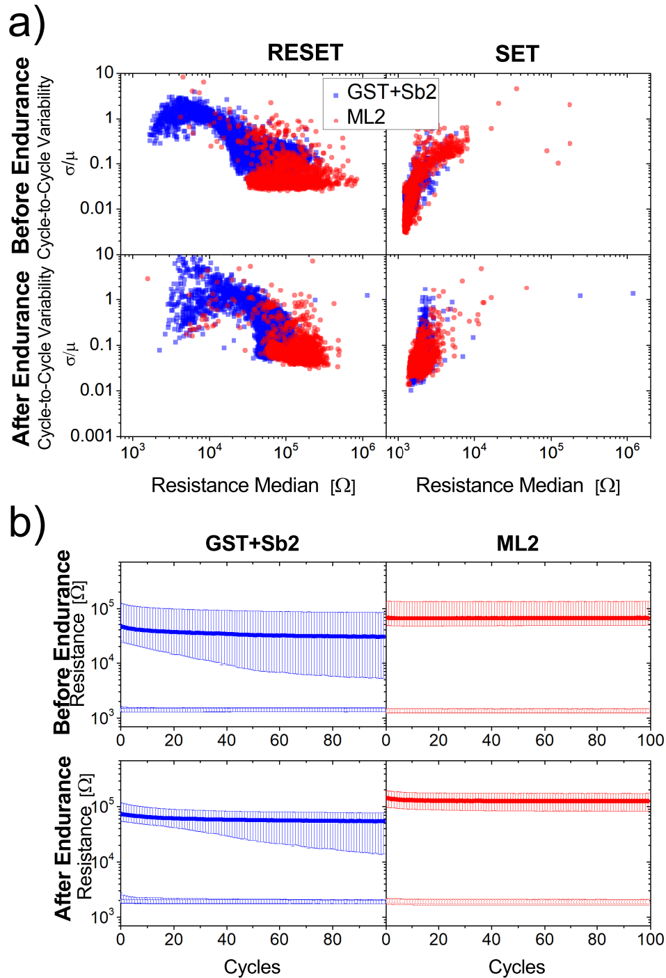
Fig. 4.12. Variability of the SET and RESET states evaluated along 100 programming cycles (SET/RESET pulses of 50 ns) in 4kb arrays, before and after a sequence of 10^3 cycles (performed with 10\ \mu\text{s} SET/RESET pulses for an accelerated aging of the devices). a) cycle-to-cycle: each point in the graphs represents the variance of the resistance value (for both RESET and SET state) of a single device normalized with respect to its median resistance along 100 cycles. b) device-to-device: median and standard deviation for the 4kb devices resistance values along the 100 cycles.
