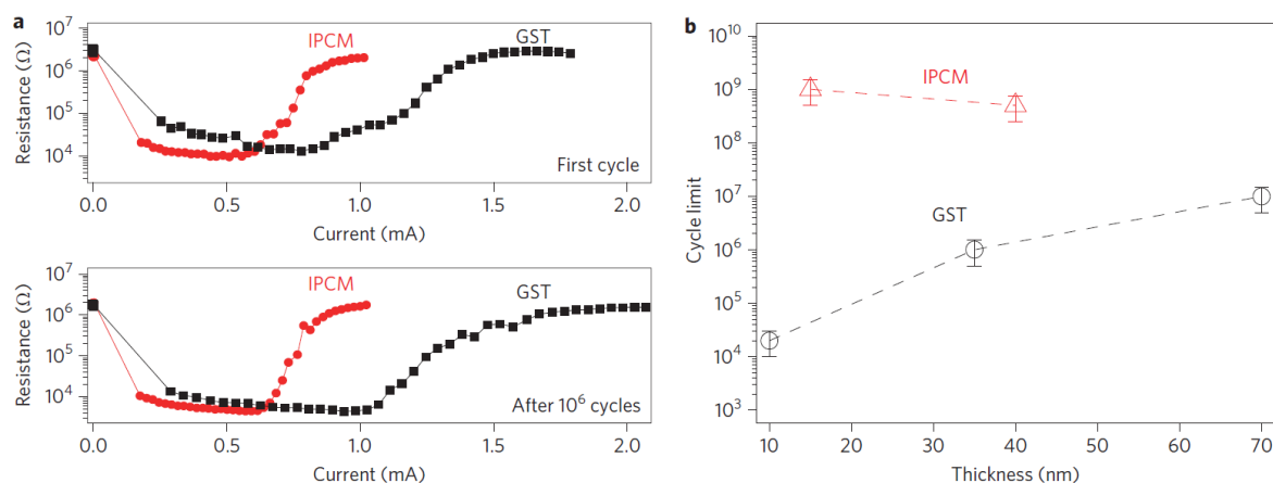
Fig. 2.23. a) R-I characteristic of IPCM devices. b) Maximum number of endurance cycles as a function of phase-change material thickness [149]
