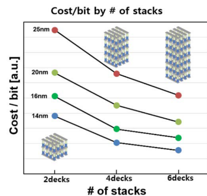
Fig. 1.9. Calculated cost per bit for scaling and vertical stack-up. [39].
