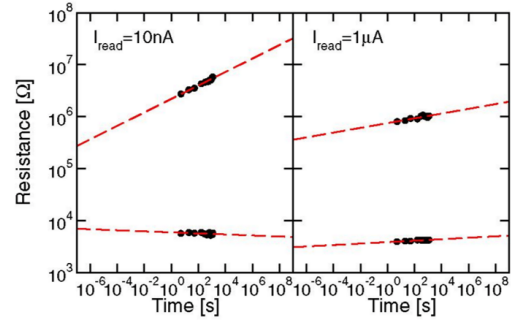
Fig. 2.12. Resistance drift for two different read currents [98].
