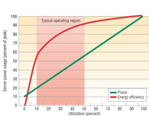
Fig. 1. Power usage and energy efficiency in a server [6].
