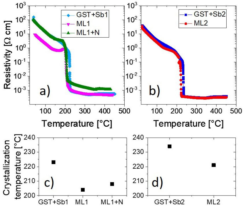
Fig. 4.2. Resistivity of as-deposited materials analyzed as a function of the temperature, measured during a ramp up of 10 ^{\circ} C/min (a-b) and their crystallization temperature (c-d).
