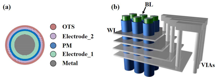
Fig. 1.11. Vertical cross-point architecture. a) Cross section of the bit-line pillar. b) Schematic of the overall vertical cross-point architecture [46].
