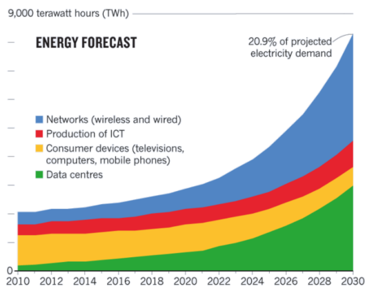
Fig. 2. Energy required by the ICT sector [9].
