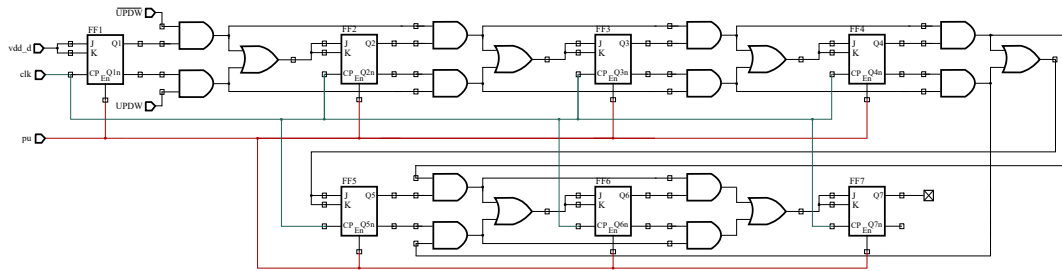
(b) Logic-gate level counter architecture: 7-bit up/down counting is realized by means of JK Flip-Flops: UPDW and UPDW inputs reverse the counting direction when toggled.
