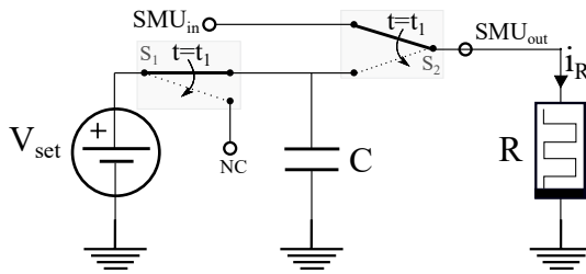
(c) Equivalent circuit
