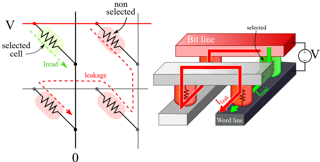
Figure 16 – Sneak paths problem in a selector-less array. Non-selected cells provide an alternative path for current, which results in a leakage contribution at the output.
