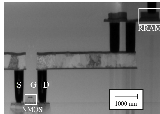
(d) TEM picture of 1T1R cell, where the RRAM is stacked on top of the transistor's drain. Adapted from [81].
