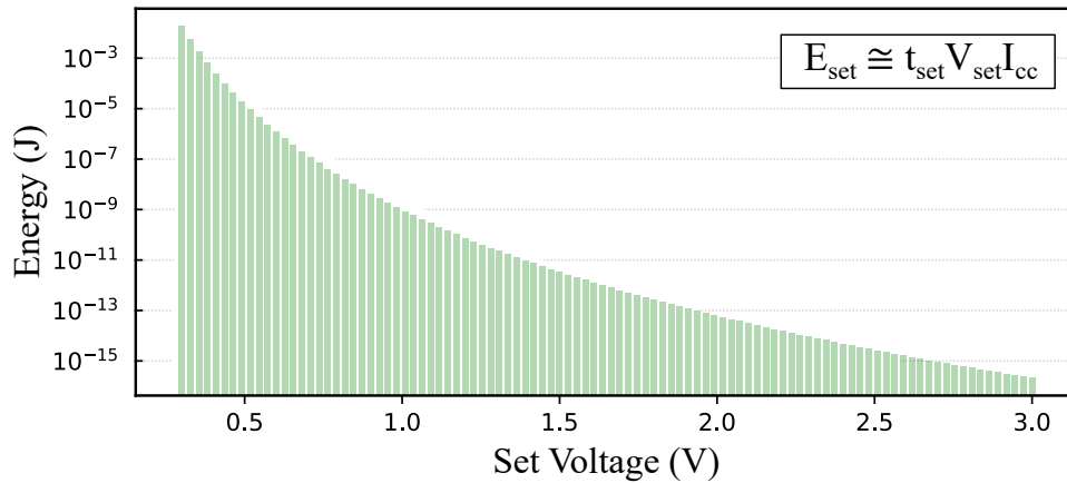
(c) Extrapolated set energy consumption versus the set voltage. The current compliance value adopted was I_{cc} = 100 \mu\text{A} . The energy cost drops as the set voltage is increased.
