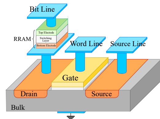
(c) 3D schematic view of the integration process of a 1T1R cell, where the RRAM element is stacked on the drain of the underlying NMOS transistor.
