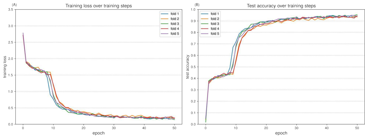
Training and test accuracy of the FFNN model
