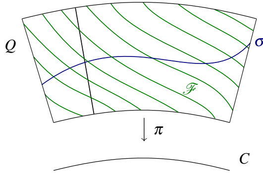
Figure 2.1 – A \mathrm{PGL}(2, \mathbb{C}) -oper on C .
