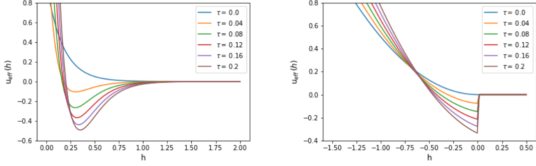
Figure 4.11: Effective pair potential for different values of \hat{\tau} for \beta = 1 and \sigma = 1 . (Left) The bare potential is taken of the form \hat{U}(h) = u_0 e^{-\lambda h} with u_0 = 1 and \lambda = 6 . (Right) The bare potential is taken of the form \hat{U}(h) = u_0 h^2 \Theta(-h)/2 with u_0 = 1 .
