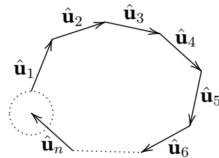
Figure 3.1: A configuration of the \hat{\mathbf{u}}_i displaying a closed loop. The dashed circle has radius less than \epsilon .
