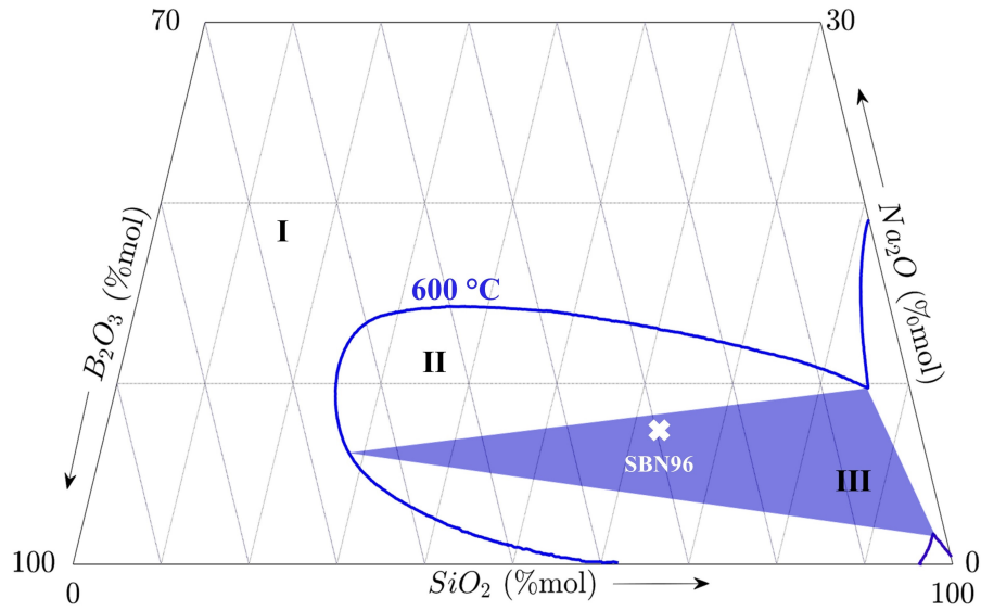
Figure III.1: Immiscibility diagram posed by Haller [106] for SBN systems at 600 °C with the location of SBN96 marked by the white cross.
