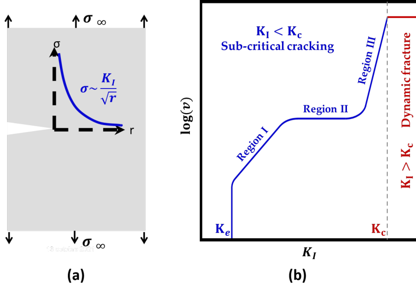
Figure 2.11: (a) Sketch of opening mode (Mode I) cracking; (b) Schematic of the log of the velocity ( \log(v) ) as a function of the stress intensity factor ( K_I ) depicting the three regions of sub-critical cracking ( K_I < K_C ).
