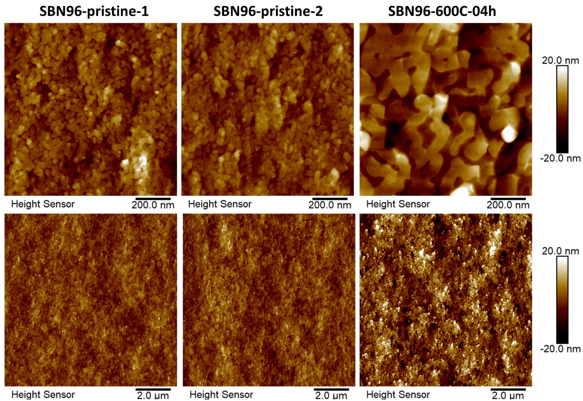
Figure III-2.3: AFM height sensor images on the fracture surfaces of SBN96 samples of size 1 \times 1 \mu\text{m}^2 for the first row and 10 \times 10 \mu\text{m}^2 for the second row. The color bars remain the same for each row.
