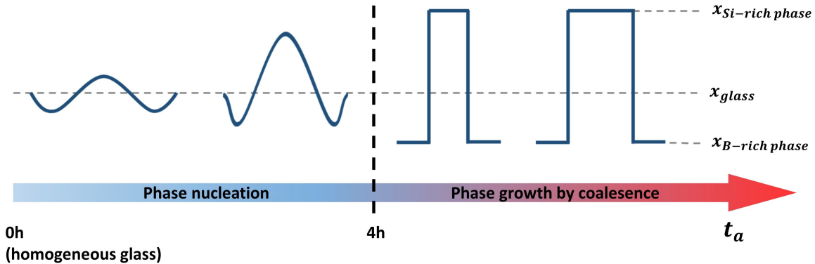
Figure III-4.1: Schematic of the evolution of concentration profiles of phases for SBN42 spinodal decomposition [7, 263].
