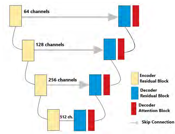
Figure 5.6: An illustration of our encoder decoder network with residual blocks, and attention.
