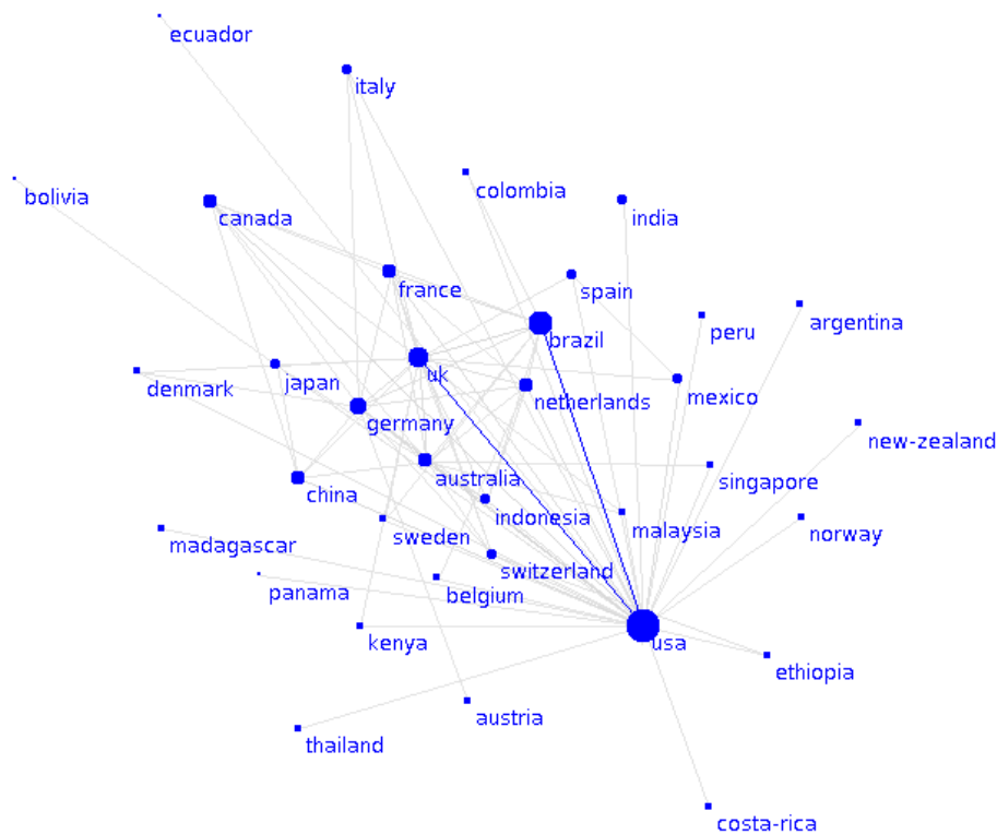
Figure 3.7: For the period from 1975 to 2016, the countries that collaborated the most with the United States were Brazil, the United Kingdom and Germany, as shown by the collaborative network around the United States.
