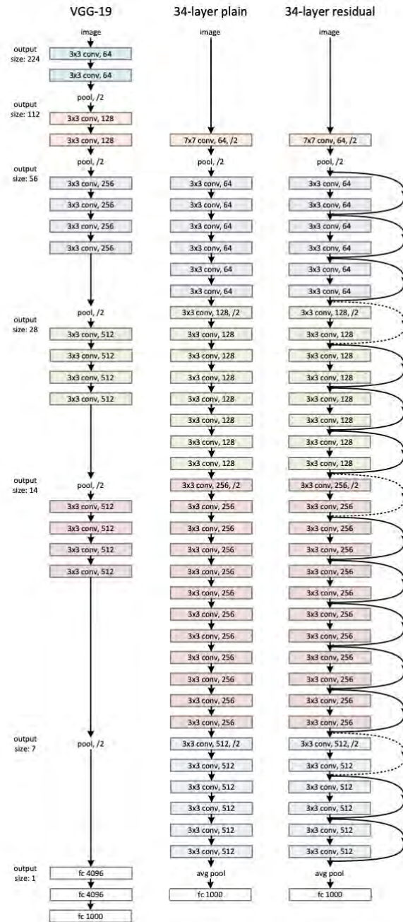
Figure 5.4: By adding skip connections to a plain 34 layer network, ResNet34 avoids training issues that occur in very deep networks. The architectures of VGG19 and ResNet34 are illustrated along with a plain 34 layer network for comparison. Skip connections are shown in ResNet34, the dotted connection increase dimensions. (Illustration from [He 2016]).
