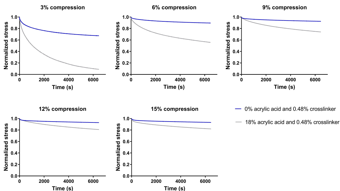
FIGURE 5.5 – Normalized stress relaxation of two hydrogels with 0.48% of crosslinker and 0 or 18% of acrylic acid as a function of time (6480 s) at different compression stages. The relaxation extent is higher for a gel with 18% acrylic acid compared to a pure polyacrylamide gel.
