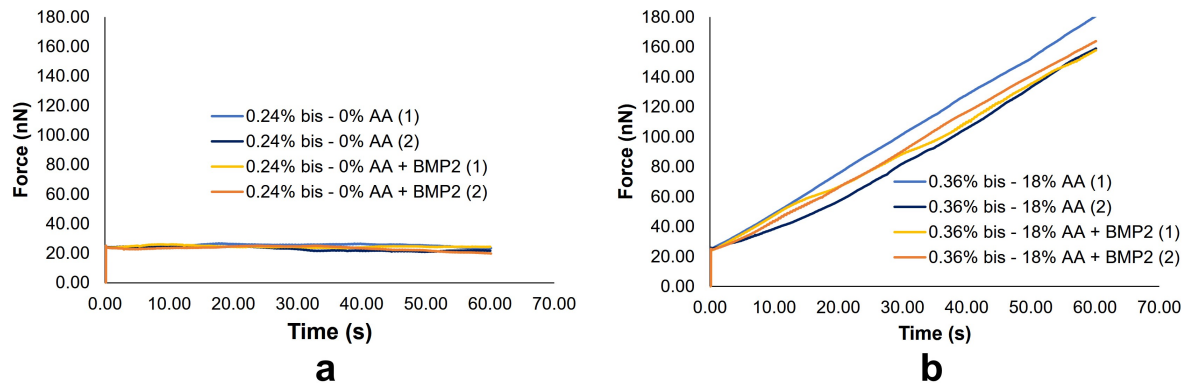
FIGURE 6.4 – Examples of stress relaxation curves of a) a pure polyacrylamide gel (15% relaxation in compression) and b) a gel containing 18% acrylic acid (70% relaxation in compression), with and without surface functionalization, measured at different locations on the sample using AFM. The behavior of the two hydrogel formulations is drastically different, and the stress relaxation is not affected by the surface functionalization with the BMP-2 mimetic peptide. (bis = bis-acrylamide, i.e., the crosslinker, AA = acrylic acid)
