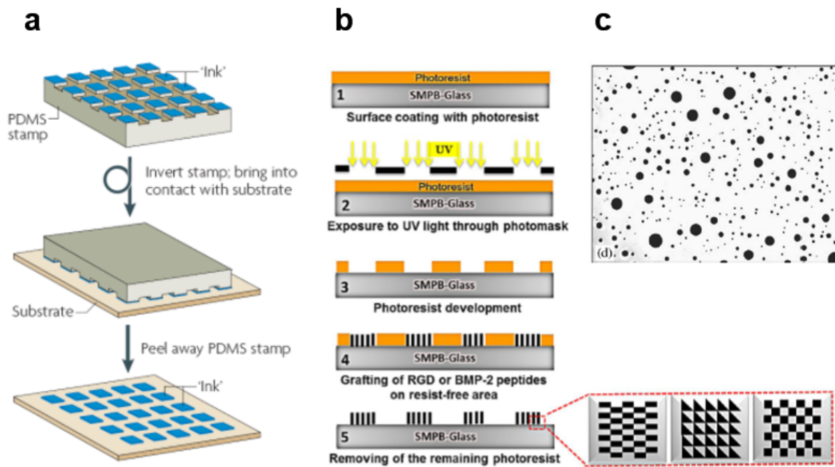
FIGURE 7.8 – a) Schematic representation of soft-lithography. b) Schematic representation of peptide micropatterning onto glass surfaces using photolithography technique. From [103]. c) Example of peptide patterning of a polytetrafluoroethylene surface using aerosols. From [387]
