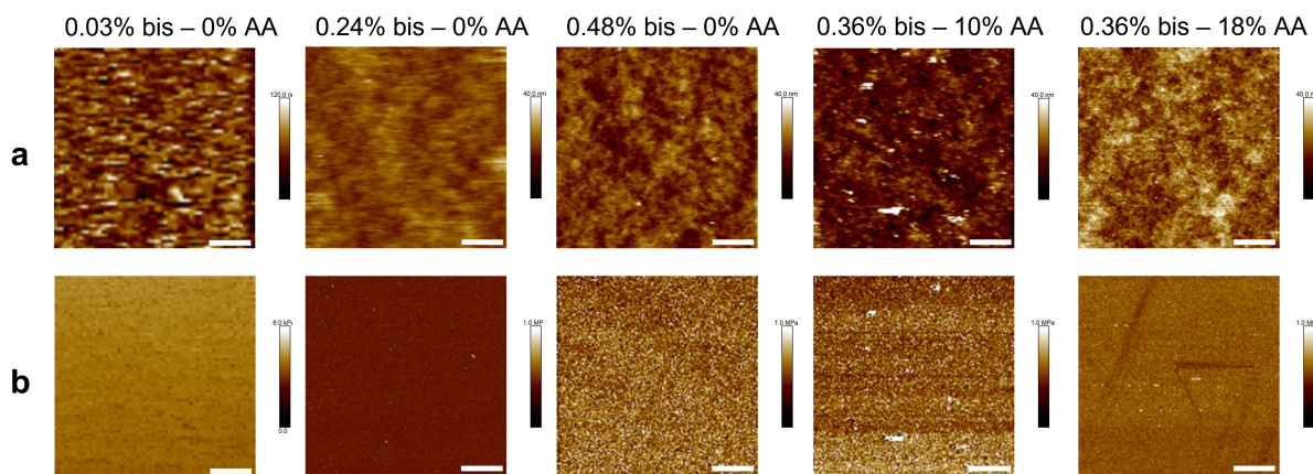
FIGURE 6.10 – a) AFM images of the surface topography on different hydrogel formulations after surface functionalization with a BMP-2 mimetic peptide. Scale bar = 8 \mu\text{m} . b) AFM indentation map on a 40 \mu\text{m} x 40 \mu\text{m} area of five polyacrylamide based hydrogels with varying formulation after surface functionalization with a BMP-2 mimetic peptide. The color bar represents the elastic modulus (Young's modulus). The surface topography is similar between the different hydrogel formulations. The surface elastic modulus is highly homogeneous for all the hydrogel formulations. In addition, the surface roughness (arithmetic mean roughness R_a ) of the hydrogels after the functionalization has been evaluated between 2.1 \pm 0.5 nm and 3.4 \pm 0.6 nm. Therefore, the roughness of the functionalized hydrogels is similar, which excludes that differences in cell behavior on the different hydrogels could be attributed to differences in surface roughness. (bis = bis-acrylamide, i.e., the crosslinker, AA = acrylic acid)
