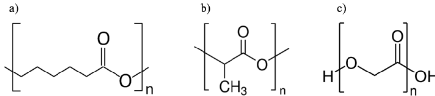
FIGURE 1.9 – Synthetic degradable polymeric materials investigated for use in bone repair. Chemical structure of a) poly( \epsilon -caprolactone) (PCL), b) polylactic acid (PLA), and c) polyglycolic acid (PGA).
