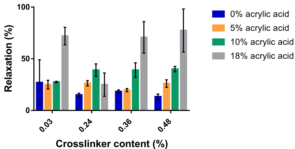
FIGURE 5.6 – Total stress relaxation for the different hydrogel formulations as a function of the crosslinker content at 6% compression. The relaxation increases with the amount of acrylic acid. (n=3)
