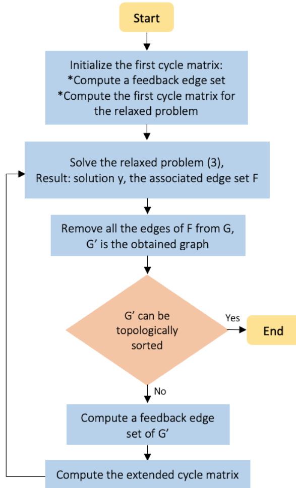
Figure 5.3: Overview of the FAS algorithm
