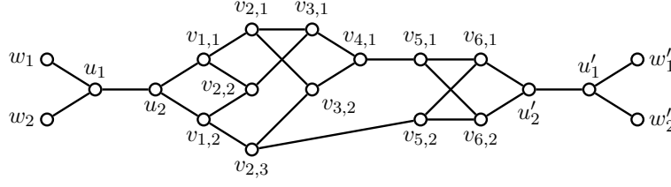
Figure A.1: The gadget used in the construction of Theorem 7.10
