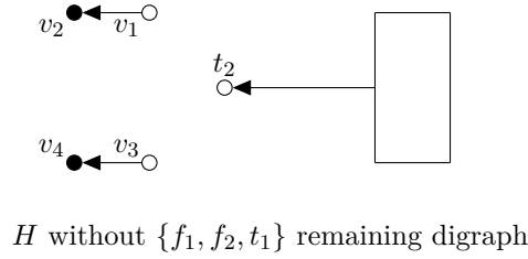
Figure 6.3: For the remaining digraph, it has been proved that is acyclic in the previous theorem so \{f_1, f_2, t_1\} is a directed feedback vertex set of the whole digraph.
