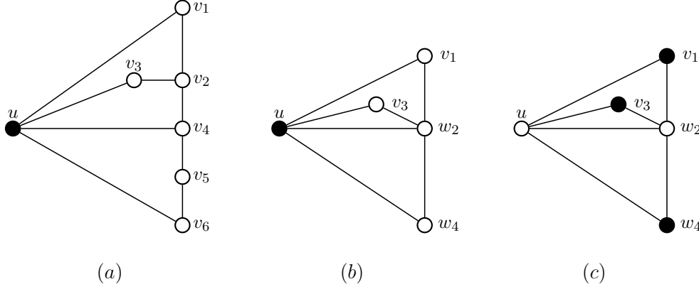
Figure 5.1: (a) vertex u is a minimal fvs of the given graph and has 4 neighbors in G[F] . (b) a contracted form of G[F] with 4 vertices. (c) a new minimal fvs of the result graph of size 3.
