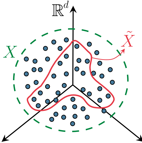
Figure 5.3: Diagram of the idea behind the Nyström approximation. A subset \tilde{\mathbf{X}} of points is chosen from the full dataset \mathbf{X} to perform the matrix calculations. The subset of points has to represent the properties of the full dataset, so they need to be chosen properly to avoid over-representing certain features.
