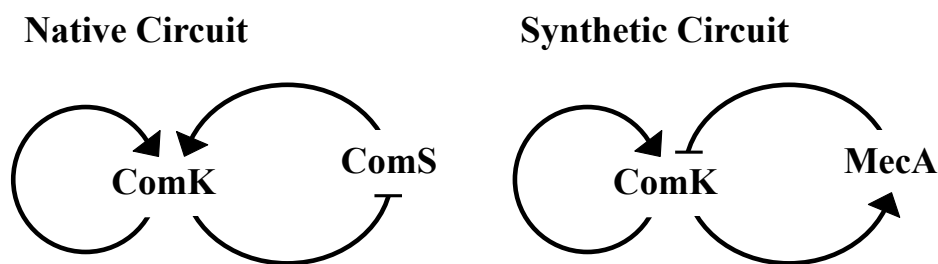
Figure 3: Endogenous regulation of ComK vs. an alternatively engineered synthetic circuit
