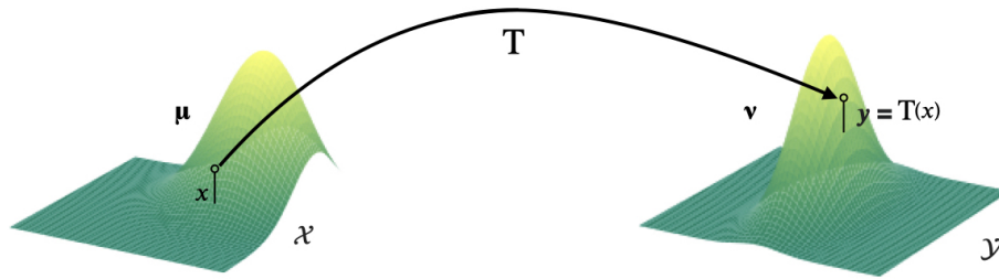
FIGURE 2.1: Illustration of Monge's problem: T is a transport map from \mathcal{X} to \mathcal{Y} .
