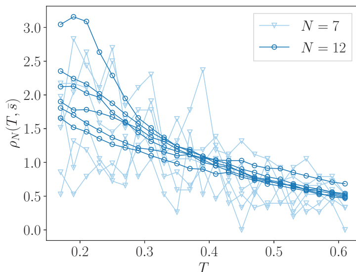
Figure 2.31: Density of change \rho_N(T, \bar{s}) as a function of T for several targets of size 7 and 12 (each curve corresponds to a different target). The step in the temperature is \Delta T = 0.02 .
