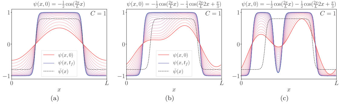
Figure 4.19: Illustration of the phenomenon of interaction of modes and the impact of the dominant mode in the morphology, for C = 1 and t_f = 5t_c . (a) The dynamics of the largest mode, alone, leads to a symmetrical final profile with the same period of the initial condition. (b) Disruptive addition of the second mode. By interaction, the final profile is no longer symmetric and is slightly shifted with respect to the initial position of the first mode. (c) As the amplitude of the second mode increases, its contribution to the dynamics of the system becomes more important, and the final profile can have the same period as the initial condition (the legend has been omitted for visualization purposes).
