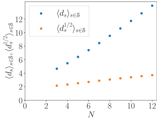
Figure 2.10: Mean of the degrees of the states d_s and their square roots over all states, for clusters of increasing size.
