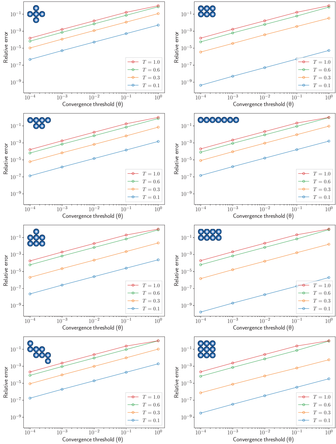
Figure A.6: Relative error of the accuracy of the value iteration algorithm as a function of the convergence threshold \theta , for some targets with N \leq 9 .
