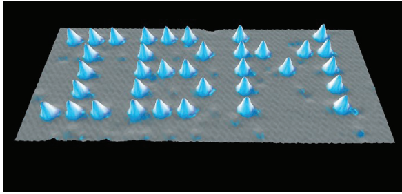
(a) Xe atoms arranged on a Ni substrate at 4 K to form the letters IBM. Each letter is 40 Å from top to bottom. Image from Ref. [7].
