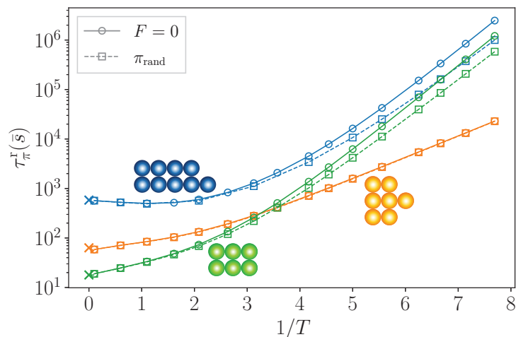
Figure 2.15: Comparison of the expected return time to target \tau_{\pi}^r(\bar{s}) for the zero-force case and under a random policy \pi_{\text{rand}} , with F_0 = 0.4 (i.e. a policy that chooses a random force with equal probability in each state) for the three targets shown in the figure, as a function of 1/T .
