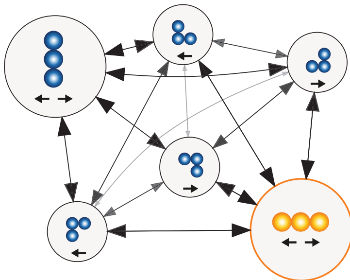
Figure 2.22: Trimer dynamics with the optimal policy computed at T = 0.61 to reach the orange target. In the target and in the upper left state, the optimal action is degenerate, and the force can be equivalently set to the right or left.
