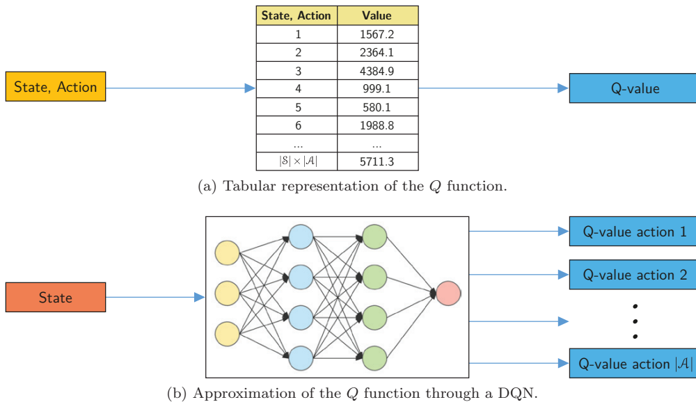
Figure 1.10: Differences in the management of the Q function according to the sizes of the state space and the action space. (a) When these spaces are of reasonable size, the Q function can be modelled by an array of dimensions |\mathcal{S}| \times |\mathcal{A}| storing the values of the state-action pairs. (b) When the dimension of one of the two spaces (or both) is too large, it is possible to use an approximation function such as a DQN, which returns, for a given state, the set of values of the different associated state/action pairs.
