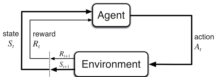
Figure 1.6: The agent-environment interface in a Markov decision process. Image from Ref. [57].
