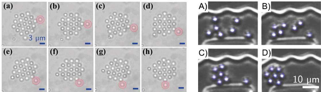
(b) Controlled rotation of colloidal clusters made of 19 silica beads (diameter \sim 2 \mu\text{m} ) with interferometric optical traps. Image from Ref. [30].
