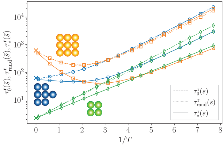
Figure 2.16: Expected return time to target as a function of 1/T . Zero-force case \tau_0^r(\bar{s}) , random-force case \tau_{\text{rand}}^r(\bar{s}) and under an optimal policy \tau_*^r(\bar{s}) , with F_0 = 0.4 . The \times symbols correspond to \tau_\infty^r(\bar{s}) .
