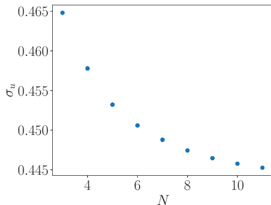
Figure 2.19: Standard deviation \sigma_u as a function of N . A fit with a decaying exponential gives an asymptotic value of \sim 0.44 .
