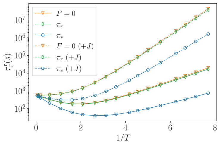
Figure A.12: Comparison of the mean return time to target as a function of inverse temperature with (dashed lines) and without (solid lines) the inclusion of an extra particle-substrate bond of energy J in the hopping energy barriers.
