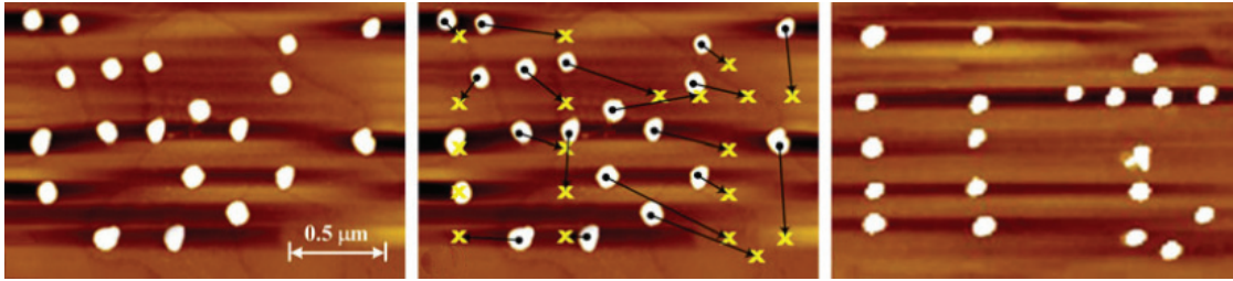
(e) Pattern composed of 20 latex nanoparticles (diameter 50 nm) on a Si substrate. Left: initial configuration, middle: pushing paths computed by the algorithm, right: final configuration. Image from Ref. [17].
