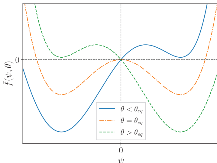
Figure 4.27: Sketch of the free energy in Eq. (4.30) above, below and at the melting temperature \theta_{\text{eq}} . The relative height of the two minima is temperature-dependent.
