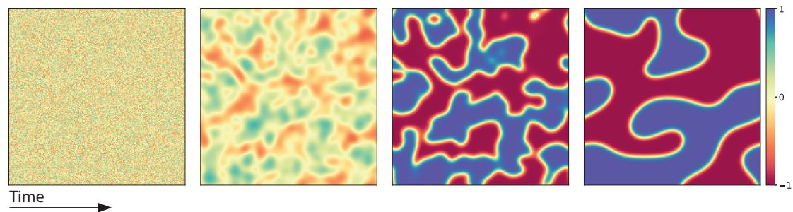
Figure 4.6: Coarsening dynamics in the two-dimensional Allen-Cahn equation with \varepsilon = 1 .
