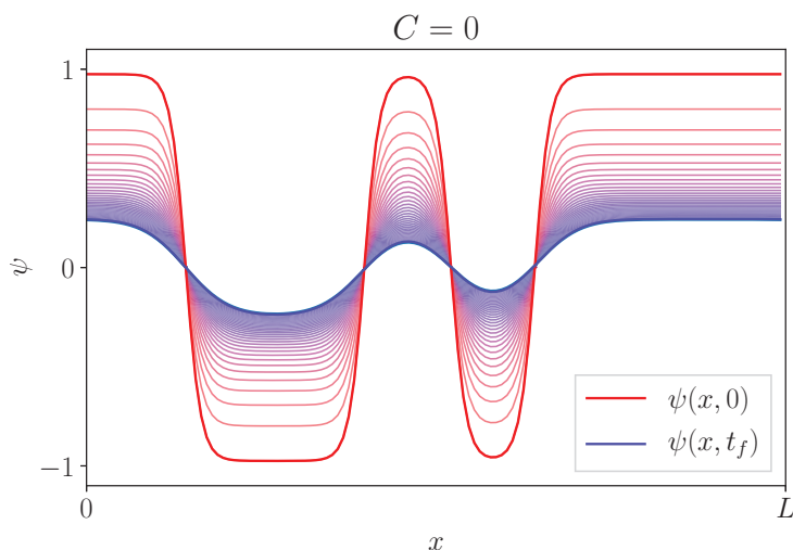
Figure 4.10: Starting from an initial profile (in red) with plateaus at amplitudes \pm C^{1/2} = \pm 1 , it is possible to reach shapes with plateaus at intermediate amplitudes by setting C = 0 or C = -1 and letting the profile relax towards \psi = 0 . Here, we have set C = 0 and a final time t_f = 8t_c .
