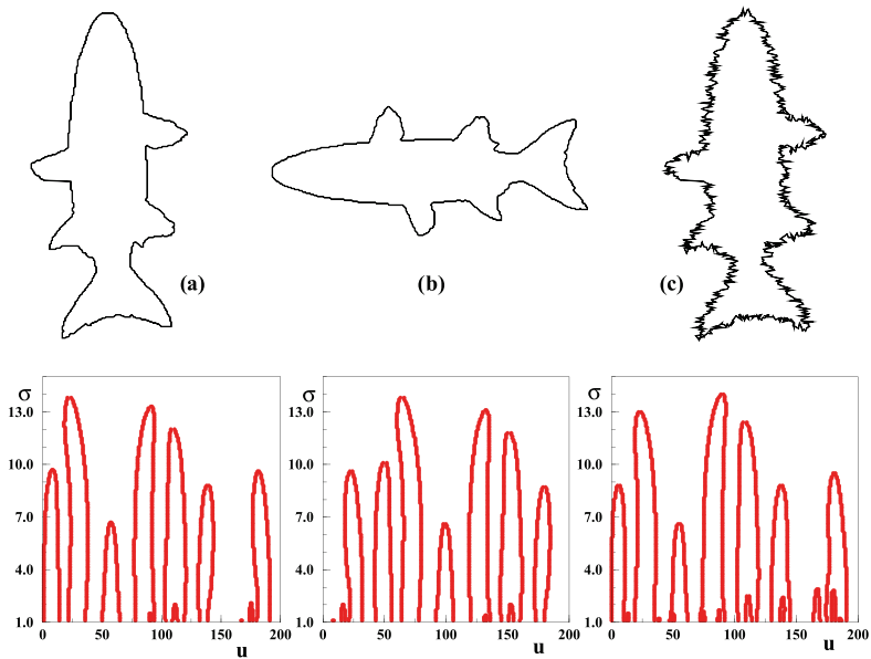
Figure 4.34: (a) A boundary and its CSS diagram. (b) Change in orientation causes a shift in the diagram. (c) Noise creates small curves at small \sigma . Image from Ref. [201].
