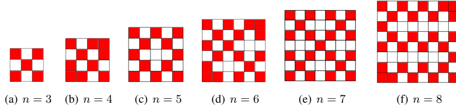
Figure 4.1 – Some instances of minimum lethal sets in G_{n \times n} when r = 3 . The vertices are depicted as small squares. Initially infected (resp., not infected) vertices are red (resp., white).
