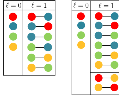
Figure 1.2 – Features induced by the 1-step random walk kernel for G_1 and G_2 , respectively.
