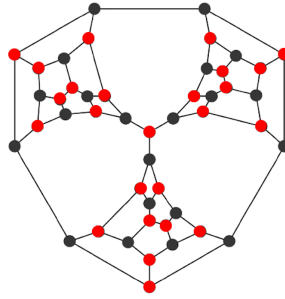
Figure 1.6 – Configuration at t = 1 for the reversible process.
