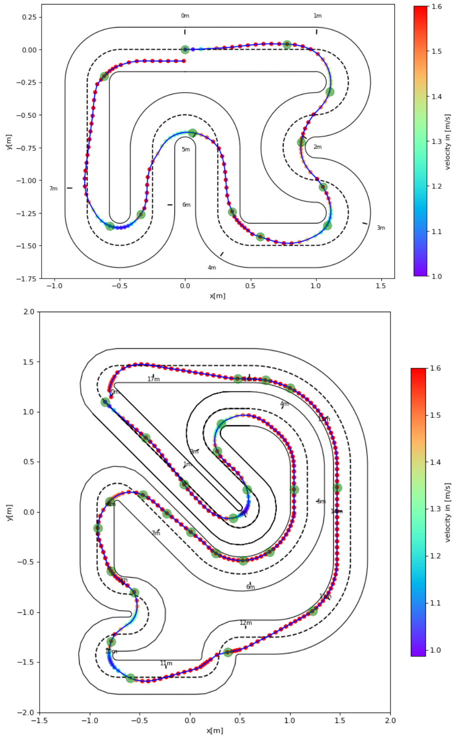
Figure 3.7: Trajectories using the triggering-based method ( N = 30 ) (Top/Down: track 1/2). Green dots represent progress points triggering-based NMPC recalculations; red points represent the baseline NMPC recalculations. Colorbars represent speed.
