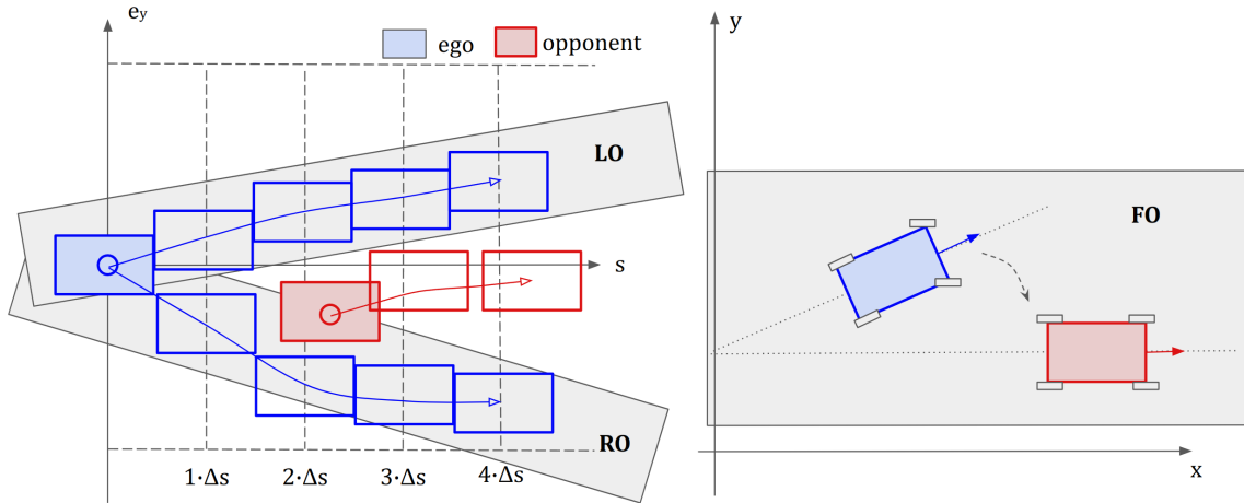
Figure 4.4: An illustrative example for the LOROFO algorithm.
