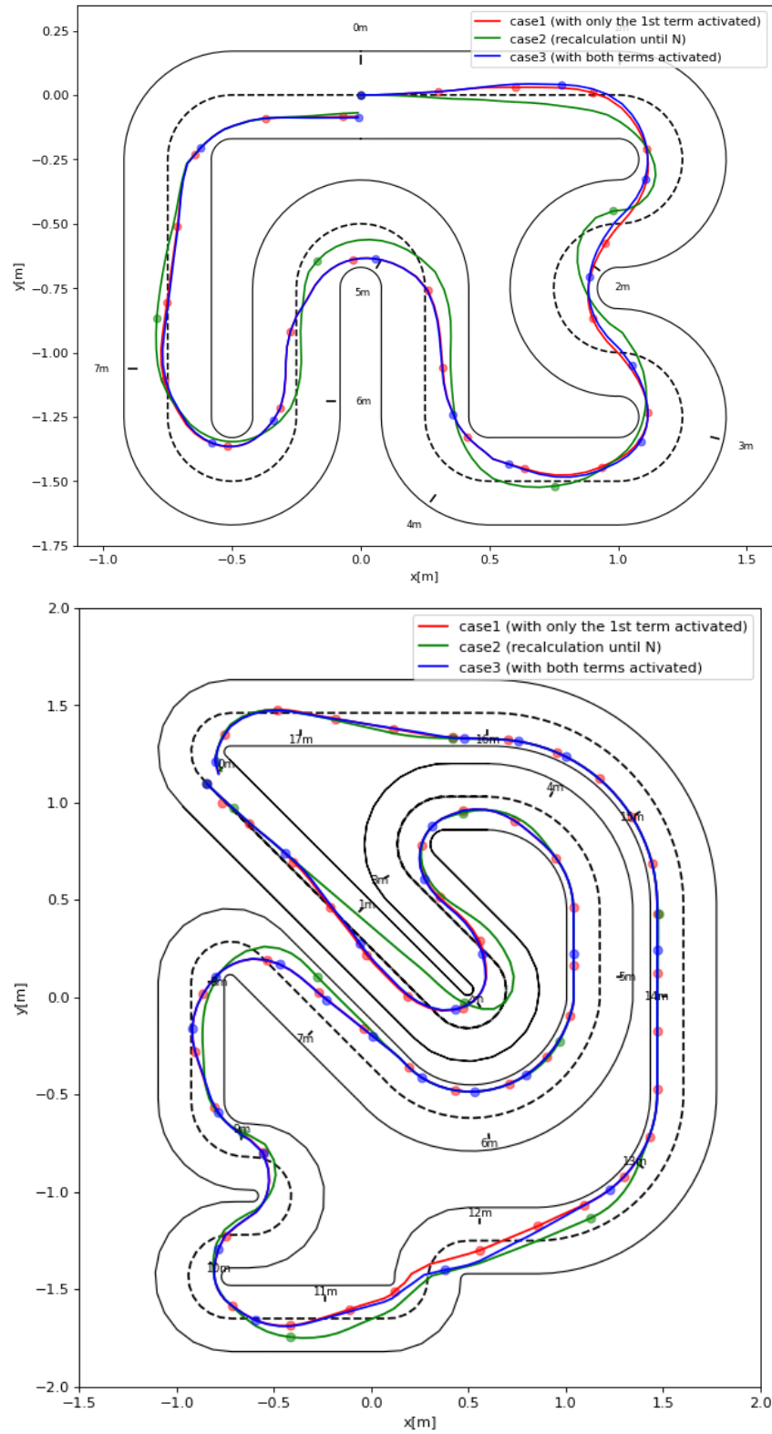
Figure 3.10: Trajectories using different configurations of the triggering conditions (Top/Down: track 1/2). Dots represent recalculations events.
