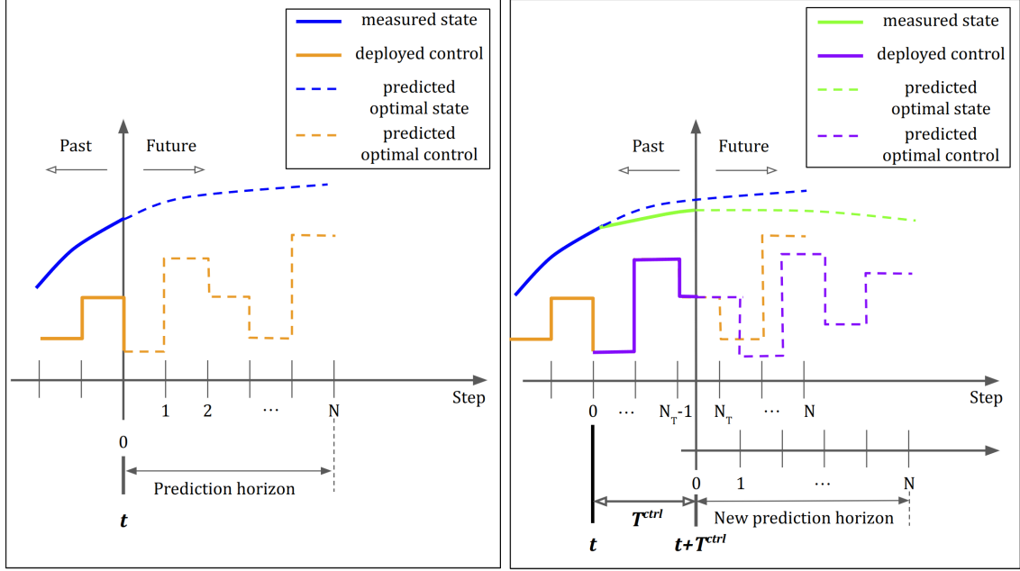
Figure 4.3: Deployment procedure for NMPC using periodic control.
