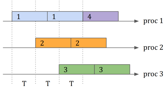
Figure 5.4: An example for \text{degree}_{DAG} = 2 and \text{degree} = 1 , on 3 available processors. Numbers on rectangles represent the release order of jobs. DAG components belonging to the same job are marked with the same color.
