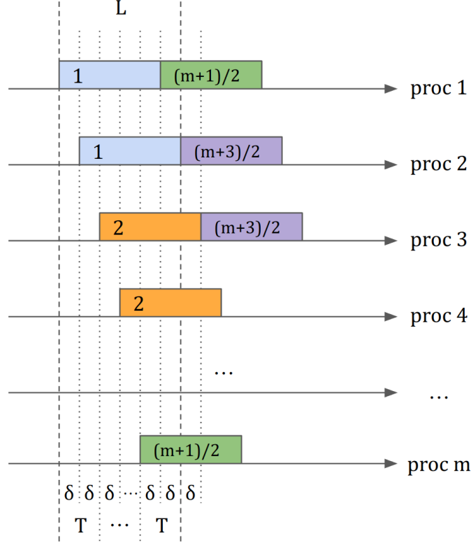
Figure 5.6: An example for \text{degree}_{DAG} = \text{degree} = 2 , on m ( m is odd) available processors. Numbers on rectangles represent the release order of jobs. DAG components belonging to the same job are marked with the same color.
