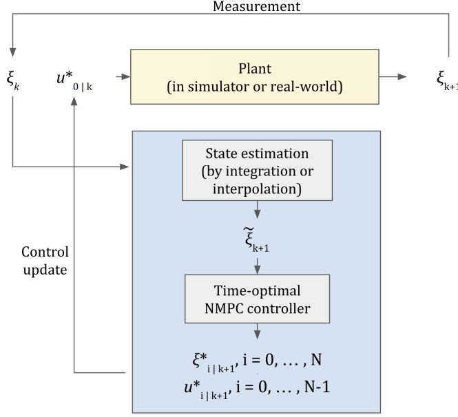
Figure 3.2: NMPC framework.
