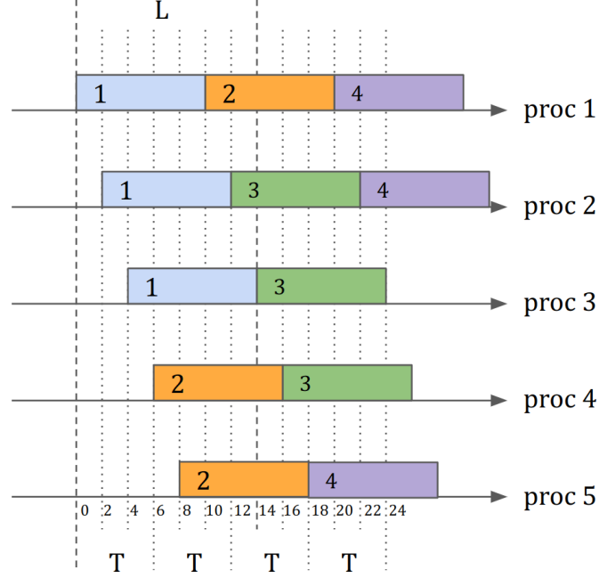
Figure 5.7: An example for degree_{DAG} = degree = 3 , on 5 processors, C = 10 . Numbers on rectangles represent the release order of jobs. DAG components belonging to the same job are marked with the same color.
