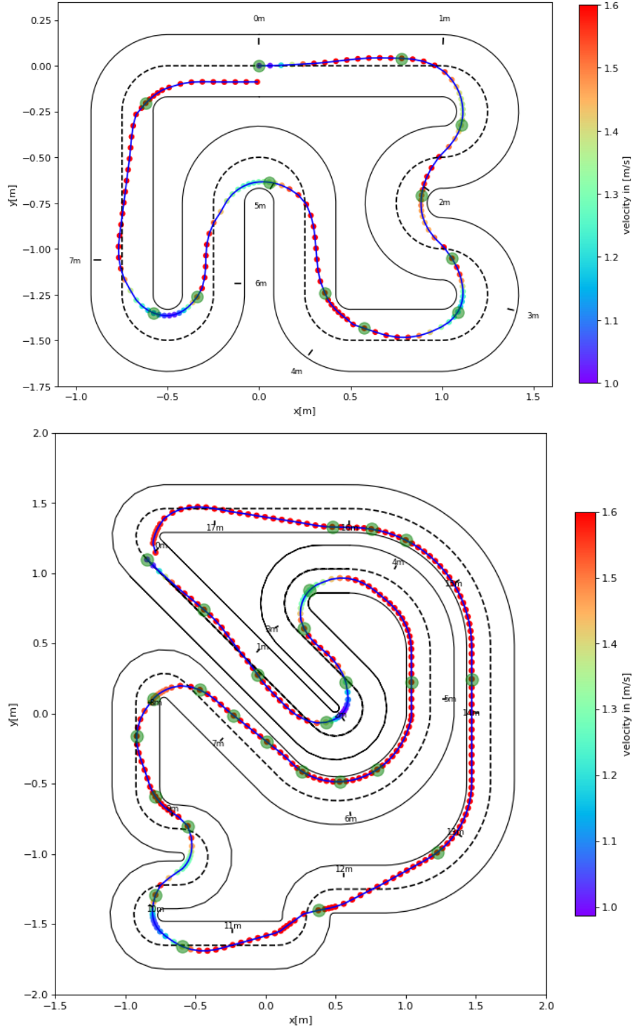
Figure 3.7: Trajectories using the triggering-based method ( N = 30 ) (Top/Down: track 1/2). Green dots represent progress points triggering-based NMPC recalculation events; red points represent the baseline NMPC recalculation events. Colorbars represent speed.
