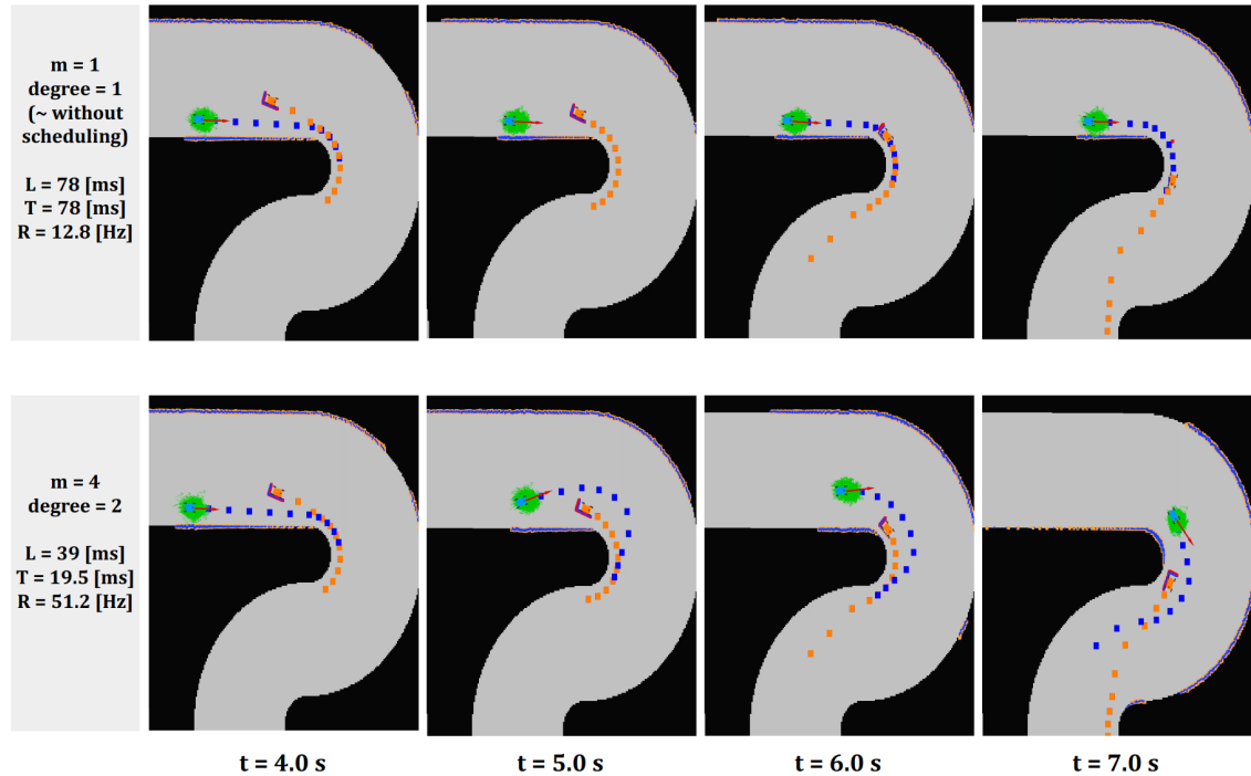
Figure 5.11: Screenshots of vehicles' pose at different time instants. Blue/orange rectangle: ego/opponent vehicle. Dot lines: planned trajectories. Green area: the collection of a large number of arrows representing the pose of each particle in PF.
