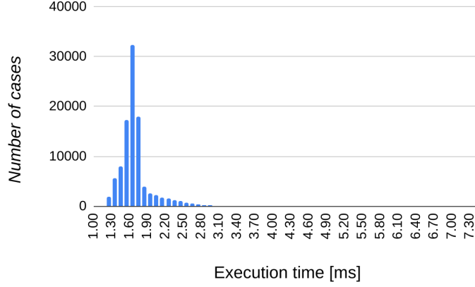
Figure 4.5: Histogram of “NMPC FW” per-iteration execution time.
