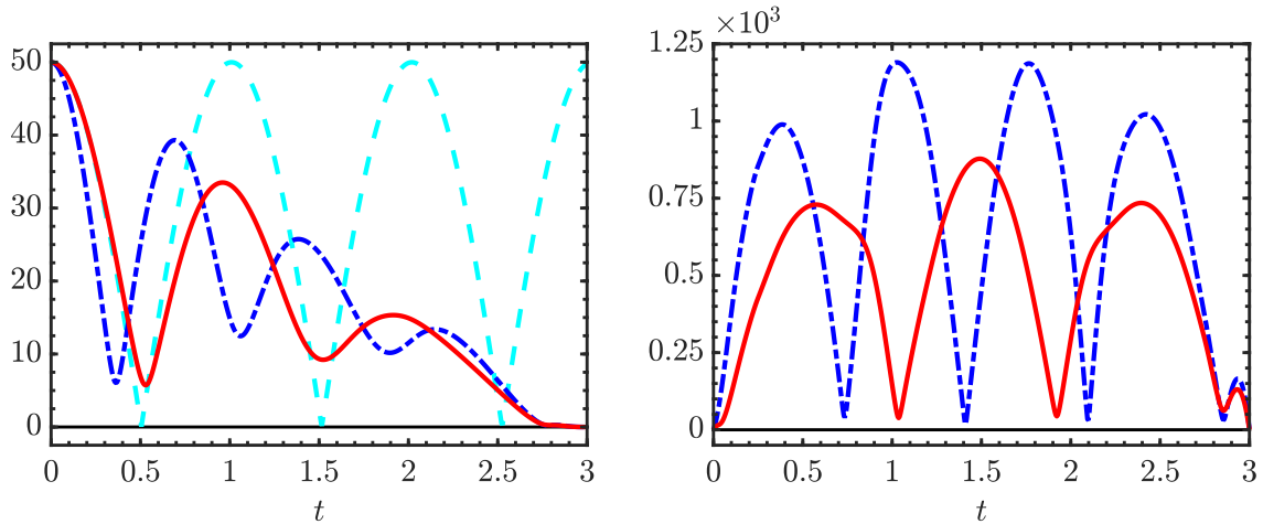
Figure 10: Fixed-point algorithm (42); c_g = 5 – Left: \|y_{k^*}(\cdot, t)\|_{L^2(\Omega)} (—) and \|y_0(\cdot, t)\|_{L^2(\Omega)} (---) vs t ; Right: \|f_{k^*}(\cdot, t)\|_{L^2_\chi(\omega)} (—) and \|f_0(\cdot, t)\|_{L^2_\chi(\omega)} (---) vs t .
