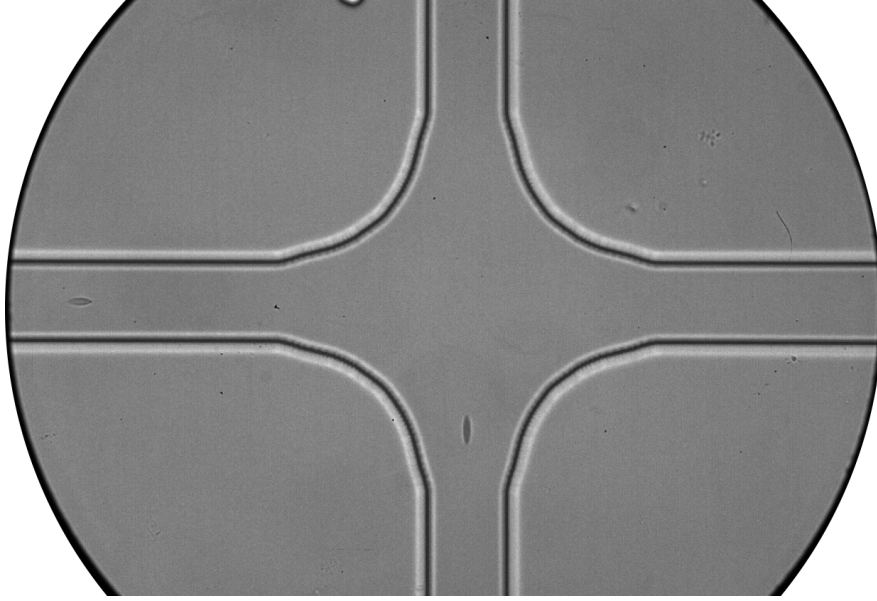
Figure 4.14: Photo of the crossflow device in operation. The horizontal channel is the input channel for the RBCs, a RBC is visible in the channel to the left of the image. An RBC after passing through the strain zone is visible at the bottom of the image, towards the exit channel.
