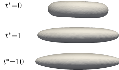
Figure 4.13: Visualization of the RBC shape at different t^* for the second orientation computation, at Ca = 0.25 and Bq_{int} = 0 .
