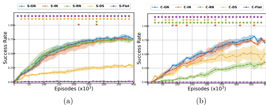
Figure 4.4: Global SR across training episodes with (a) Semantic (S) goals and (b) Continuous (C) goals for the considered agents. Mean \pm standard deviations are computed over 5 seeds. Stars highlight statistical differences w.r.t S-GN agents (Welch’s t-test with null hypothesis \mathcal{H}_0 : no difference in the means, \alpha = 0.05 ).
