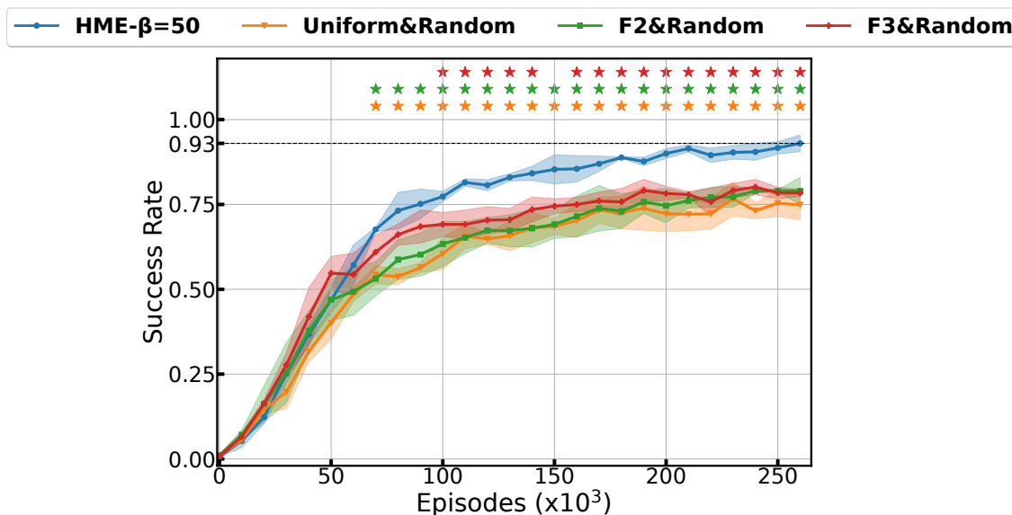
Figure 6.5: Global SR for different exploration techniques across training episodes.
