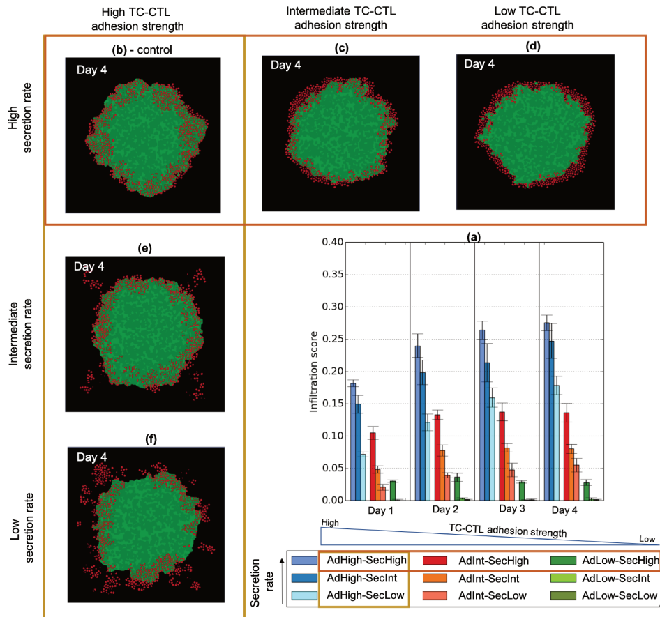
Figure 5.6: Decreasing the secretion rate of the chemoattractant and the TC-CTL adhesion strength reduce the infiltration of CTLs into the tumour. Plot in panel (a) displays the average value of the infiltration score, computed via (5.2), for different combined values of the secretion rate of the chemoattractant and the TC-CTL adhesion strength, at different times of the simulation. The error lines represent the standard deviation between 5 simulations. Inset in panel (b) displays an example of the spatial distribution of tumour cells and CTLs at the end of numerical simulations for the parameter values considered in the control scenario. Insets in panels (c)-(d) display similar plots for 2 decreasing values of the TC-CTL adhesion strength. Insets in panels (e)-(f) display similar plots for 2 decreasing values of the secretion rate of the chemoattractant.
