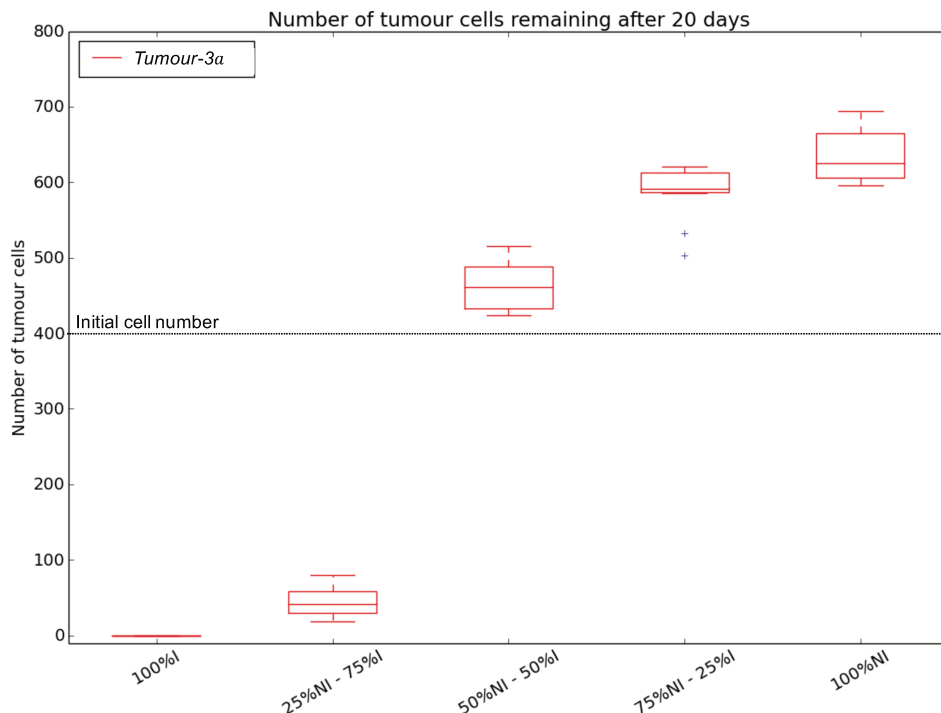
Figure 3.7: Different initial percentages of immunogenic and non-immunogenic cells can cause variations in the immune response to tumour cells. Plot displaying the number of tumour cells remaining after 20 days (28800 time-steps) for different initial percentages of immunogenic and non-immunogenic cells. For these simulations, only tumour-3a was considered. The tumour cell numbers presented here were obtained as the average over 10 simulations and the error bars display the related standard deviation. The black dotted line highlights the number of tumour cell at the initial time of the simulations.
