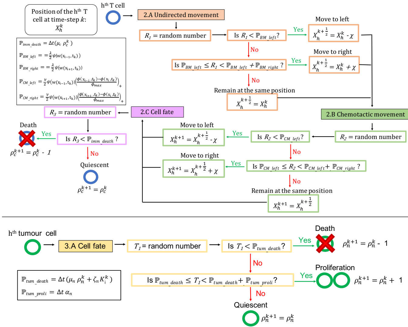
Figure D.2: Flowchart illustrating the detailed computational procedure followed to update the positions of every CTL, as well as the fate of each tumour cell and CTL in 1D. Analogous strategies are then used in a two-dimensional domain.
