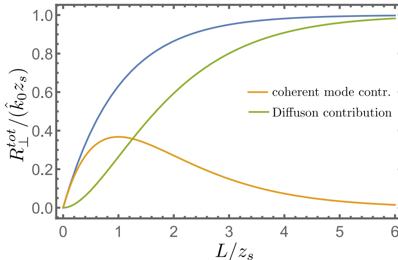
Figure 5.2: Blue curve: total beam centroid |\mathbf{R}_\perp^{\text{tot}}(L)| vs. L/z_s in the paraxial regime, Eq. (5.32). The orange and green curves, instead, stand for the contributions to |\mathbf{R}_\perp^{\text{tot}}(L)| coming from the coherent mode ( L/z_s e^{-L/z_s} ) and the Diffuson ( (1 - L/z_s e^{-L/z_s} - e^{-L/z_s}) ), respectively.
