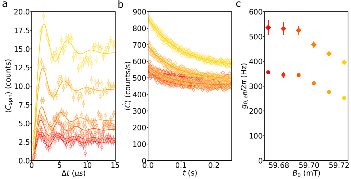
Figure 8.5: Rabi oscillations at various B_0 (setup 2) . Data measured by varying the pulse duration \Delta t at various field amplitude from B_0 = 59.673 mT (red) to B_0 = 59.723 (yellow) by step of 0.01 mT, with the parameters \varphi = 30^\circ , \beta = 11.5 \text{ ns}^{-1/2} and T_{\text{int}} = 0.075 s and T_{\text{rep}} = 0.25 s. a , Rabi oscillations (dots) fitted using Equation 8.3 (solid lines) to get g_{0,\text{eff,R}} . b , fluorescence curves at each B_0 averaged over all \Delta t (hexagons) and exponential fits yielding g_{0,\text{eff,r}} . c , effective spin coupling g_{0,\text{eff}} as a function of B_0 , fitted with the Rabi oscillation (dots) and the relaxation curves (hexagons). The error bars are 1\sigma deduced from the fits.
