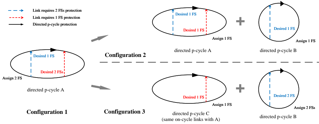
Figure 3.5: Directed p-cycle protection with different desired links.
