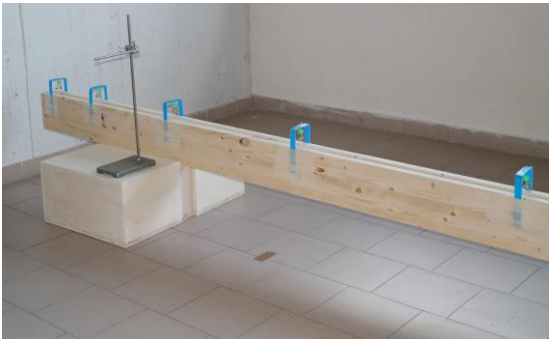
Fig. 4.12. The inclined plane with the bells and the pendulum used to verify the law of odd numbers. Source: my own experiment image.
