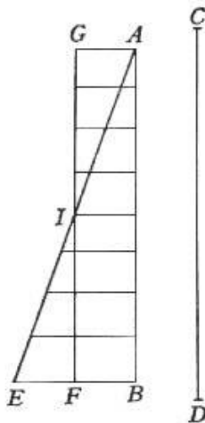
Fig. 1. Anticipating the Cartesian plane and the integral calculus, Galileo shows that the space travelled in a uniformly accelerated motion from rest represented by the area of the triangle AEB (with speeds continuously increased from A to EB) is equal to the space travelled in a uniform motion represented by the area of the rectangle GAFB (with speeds all equal to EB), distances both travelled at the same time CD. Galilei [1638], 1890-1909, vol. VIII, p. 208. Source: Bibliothèque nationale de France / gallica.bnf.fr.
