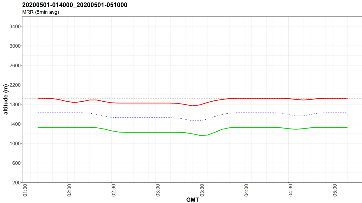
FIGURE 4.6: MRR ML time series: 1 May 2020. ML characteristics of the event observed by MRR radar. Solid red and green lines show ML top and bottom respectively. Dotted blue line shows altitude of the reflectivity peak. Dotted black line is the center of the 0^\circ beam in a PPI scan, i.e. altitude of MOUC radar. Throughout the event, the MOUC radar is in close proximity of ML top.
