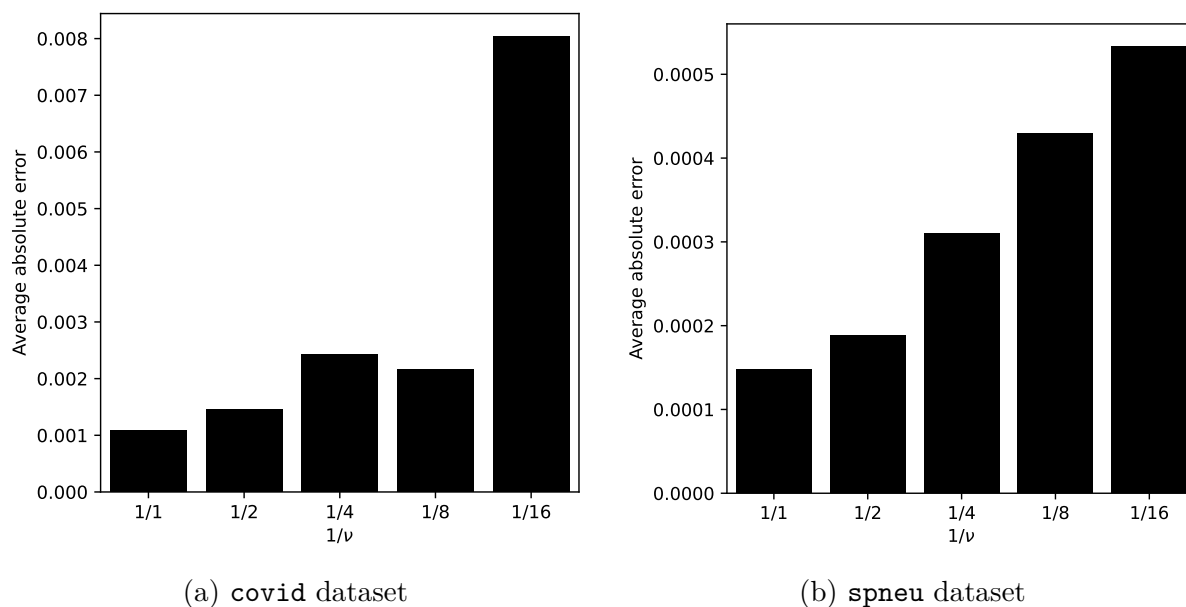
Figure 14.8: Effect of sampling syncmers before IBLT insertion on the average absolute error. 1/\nu is the compression rate used for sampling syncmer sets before IBLT insertion. \nu = 1 means no sampling (full syncmer sets).
