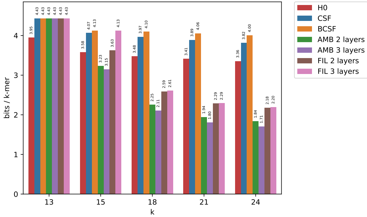
Figure 11.11: Compressed space usage for the high entropy df dataset.
