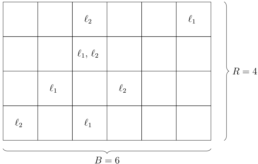
Figure 8.2: Example of a Set-Min sketch with L = \{\ell_1, \ell_2\} . Two pairs (e, \ell_1) and (f, \ell_2) with e \neq f have been inserted into the sketch, with e, f hashed to the same bucket at line 2.
