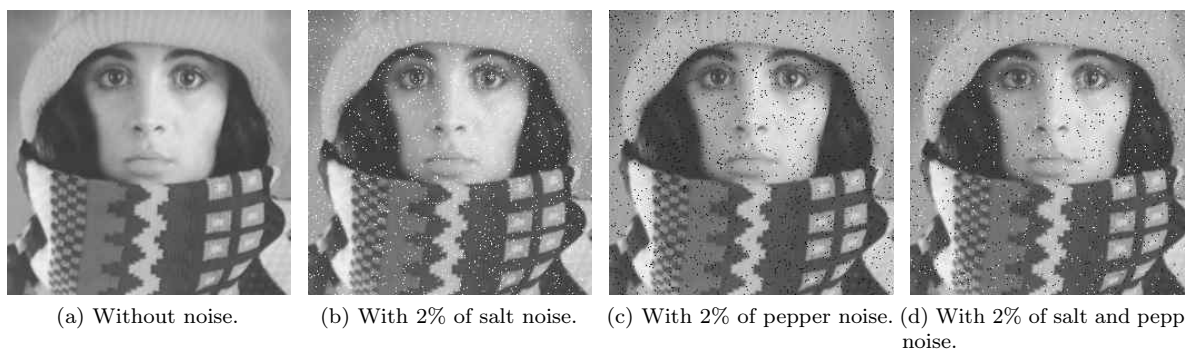
Figure 3.2: Input images.
