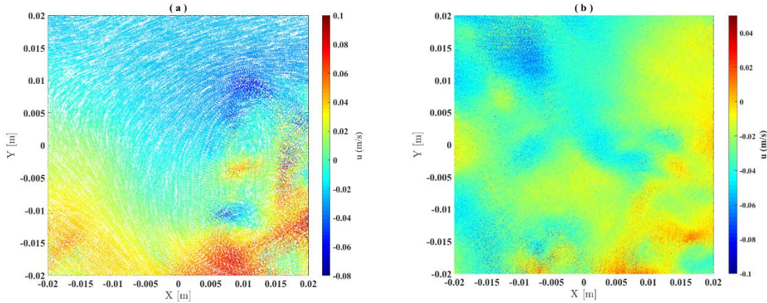
Figure III.18 2D representations of tracks for \phi_{im} = 0.05 ppp for (a) first configuration and (b) second configuration. Tracks are plotted with 10 time steps. Both are color coded with u component (velocity in x direction).
