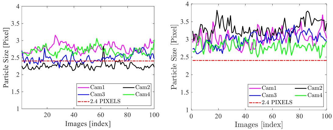
Figure III.16 Particles size for 100 random images. (Left) Spherotech (second configuration). (Right) Lavisson particles (first configuration). Particle size is estimated by fitting a 2D gaussian to the peak of correlation of one image by itself. Window size used is 64 \times 64 pixels.
