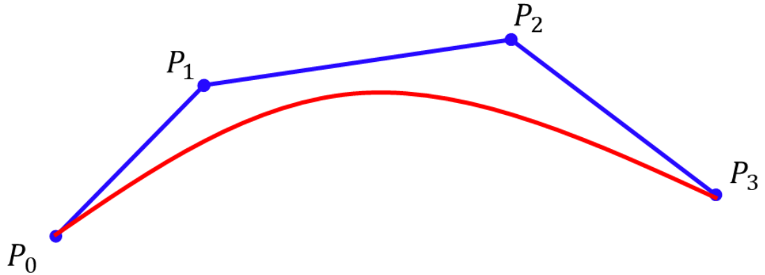
Figure II.14 Example of a cubic Bézier curve defined by four control points.
