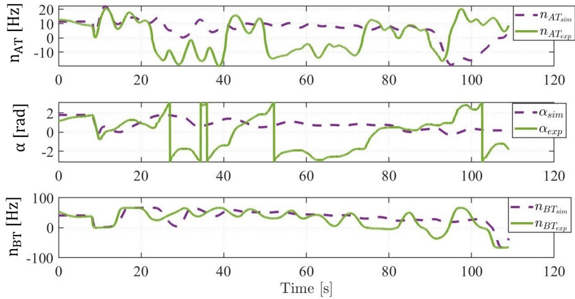
Figure 6.12: Physical inputs for initial pose \boldsymbol{\eta}_i = [33.63, 25.63, -155.27^\circ]^T .
