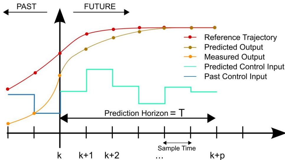
Figure 5.1: MPC scheme [94].
