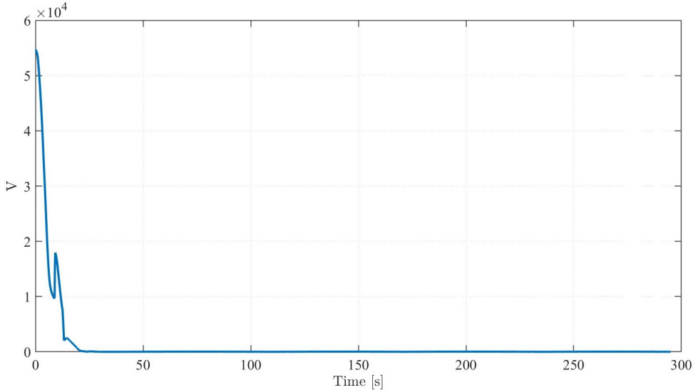
Figure 5.39: Lyapunov function value of NMPC without contraction constraint for a zig-zag maneuver.
