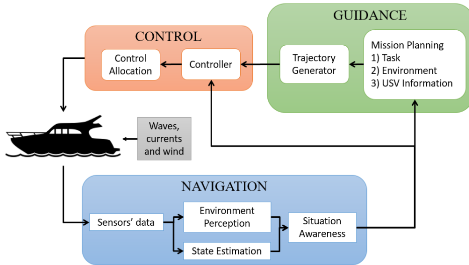
Figure 2.2: GNC system.
