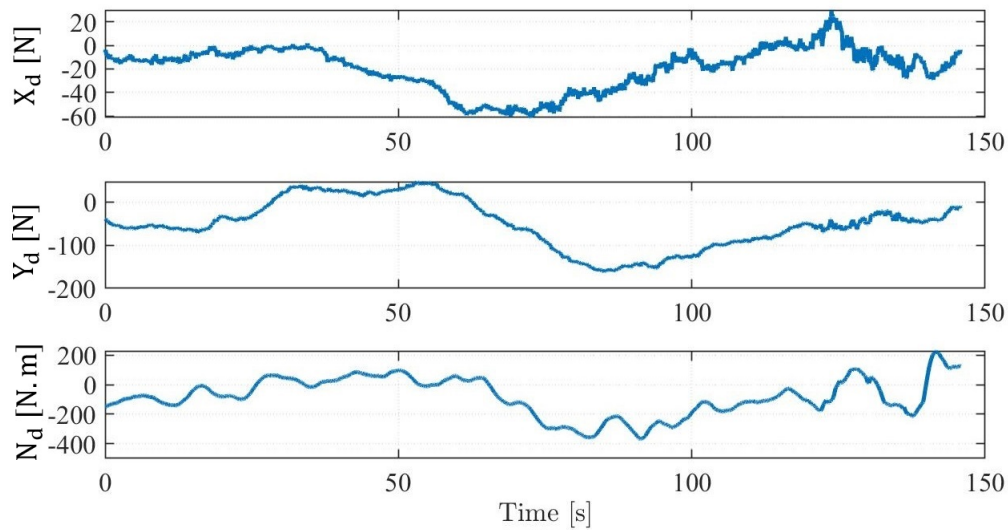
Figure 6.8: Estimated disturbances forces for initial pose \boldsymbol{\eta}_i = [-3.58, 31.92, -60.73^\circ]^T .
