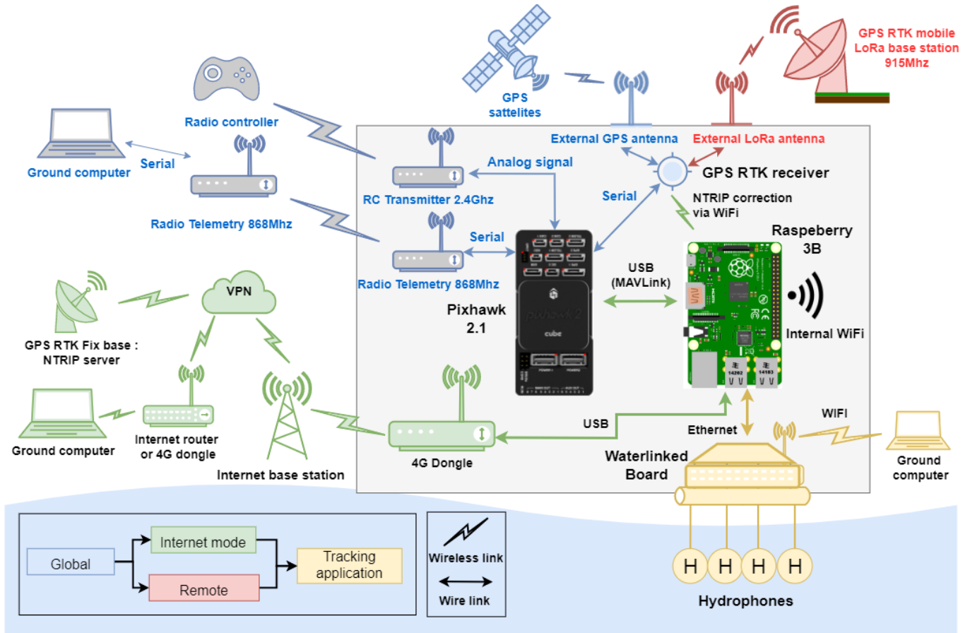
FIGURE 1.4: Network diagram of the ASV showing how the autopilot get and interact the difference sources of information to perform the navigation of the ASV
