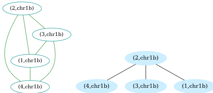
Figure 5.5 – Example 1. One expected haplotype. (Left) Similarity relations between seeds. Nodes are labeled by a number and their ground truth haplotype, and are colored according to the latter information. Edges represent similarity relations between seeds, with a color code (here, only green edges are present, i.e. all edges represent high similarity). (Right) Result of ASP phasing algorithm. Nodes are labeled as in the similarity graph. They are colored according to the phasing results: two nodes phased in the same group have the same color, and two nodes phased in different groups have different colors (the color itself does not have any meaning). Edges represent the reliability of the phasing results, as well as their consistency with the ground truth phasing. A black edge between two nodes means that these nodes are phased together both in the ground truth and in the computed phasing. A solid edge means that the phasing result is unambiguous.
