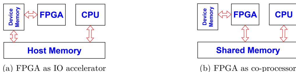
Figure 2.7 – Integration of FPGA into database systems with CPU
