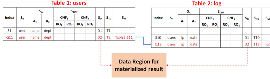
Figure 3.14 – Managing multiple semantic description tables within Multi-view processing.
