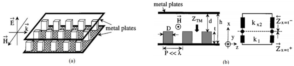
Figure 2.27: Geometry of the PBG structure. (a) periodic and regular metal posts in a PPW. (b) cross-sectional view and transverse resonance equivalent circuit of the structure [54].
