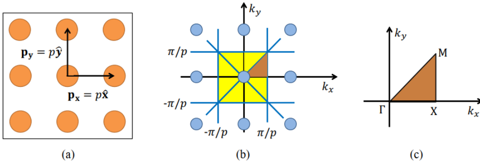
Figure 6.2: (a) Lattice vectors of a 2D periodic structure with the periodicity p along both x - and y -direction. (b) The Brillouin zone (yellow square) and the irreducible Brillouin zone (orange triangle). (c) Irreducible Brillouin zone and the conventional name of its special points.
