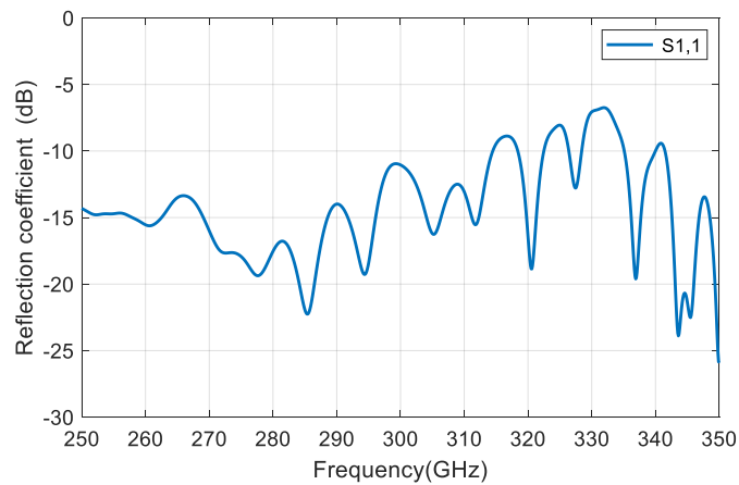
Figure 7.9: Return loss (S11) of 10.5 \lambda_0 Luneburg lens loaded with uniform metallic posts feed by a standard waveguide.
