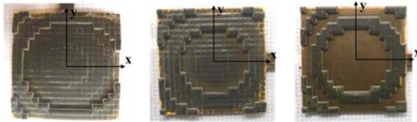
Figure 2.13: Three 3D printed reflectarrays [27].
