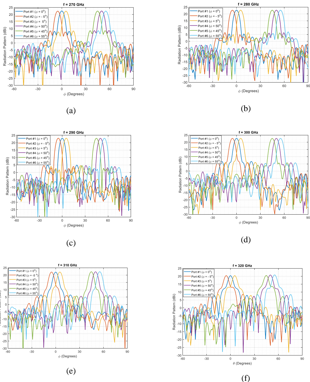
Figure 7.14: Beam steering of the 10.5 \lambda Luneburg lens antenna loaded with uniform metallic post structure.
