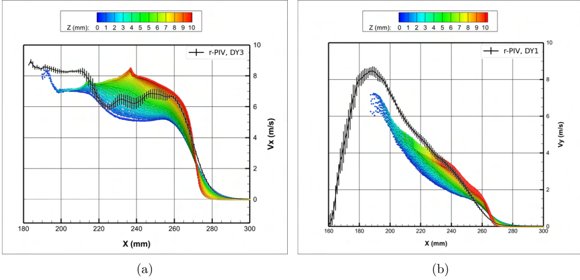
Figure 4.38 – Evolution of V_x with X between Y = -2.75\text{mm} and Y = 2.75\text{mm} (a), and V_y with X between Y = 47.5\text{mm} and Y = 52.5\text{mm} (b). The colors represent the altitude Z of the particle, and each point represents an SPH particle. We overlay the corresponding r-PIV results with the error bars representing the standard deviation between the N runs. Case Slick225 H_w = 8\text{mm} .
