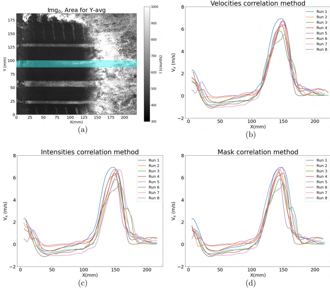
Figure 3.11 – Comparison between the three overlapping methods in the case of the PCY4 worn at V_0 = 8.33 \text{ m.s}^{-1} , H_w = 1.5 \text{ mm} and N = 8 runs. The V_x profiles of all runs are plotted Y-averaged in the area highlighted in blue in (a). Profiles obtained after using the velocities correlation method are plotted in (b), the intensities correlation in (c), and the mask correlation in (d).
