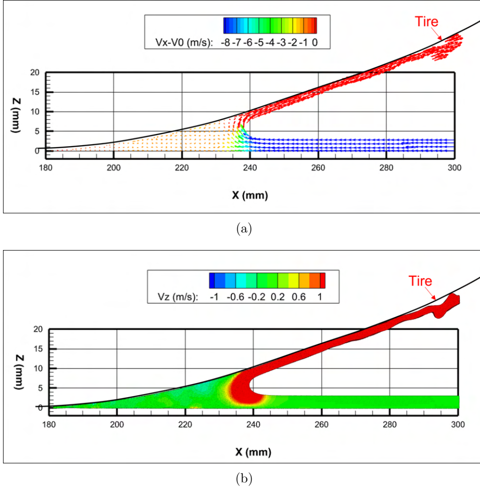
Figure 4.43 – XZ view in the middle of the WB between Y = -2.75\text{mm} and Y = 2.75\text{mm} . In (a) we represent the flow circulation with arrows in the vehicle referential, and in (b) we depict V_z . Case Slick225 H_w = 3\text{mm} .
