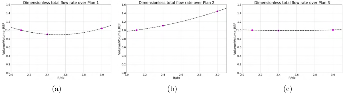
Figure 5.25 – Variation of the flow rate over P1 (left), P2 (middle) and P3 (right) for different R/\Delta x_{SPH} ratios, with a fixed SPH time step
