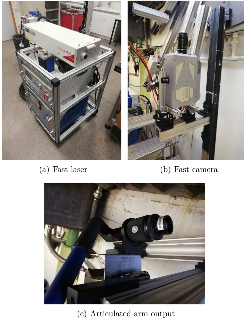
Figure 3.14 – Photos of the fast laser (upper left), the fast camera (upper right), and the optics in the output of the articulated arm (bottom)
