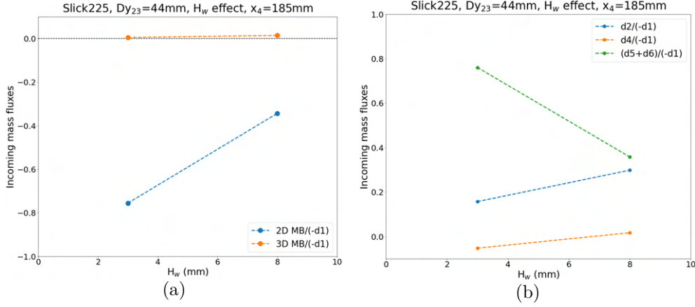
Figure 4.30 – Evolution of the 2D and 3D mass budgets profiles (a) and decomposition of the mass budget contributions on the sections S_1 to S_6 (b) for H_w = 3mm and H_w = 8mm normalized by (-d_1) , for x_4 = 185mm . The results for H_w = 8mm correspond to the Run33 and are previously presented in Fig.4.25. The results for H_w = 3mm belong to Run178.
