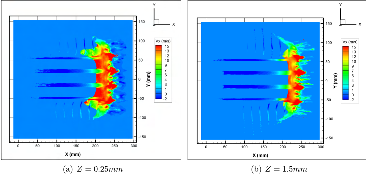
Figure 5.5 – V_x field interpolated on a slice for the PCY4 case at V_0 = 13.89m.s^{-1} and H_w = 1.5mm . On the left the slice is positioned at Z = 0.25mm and on the right at Z = 1.5mm .
