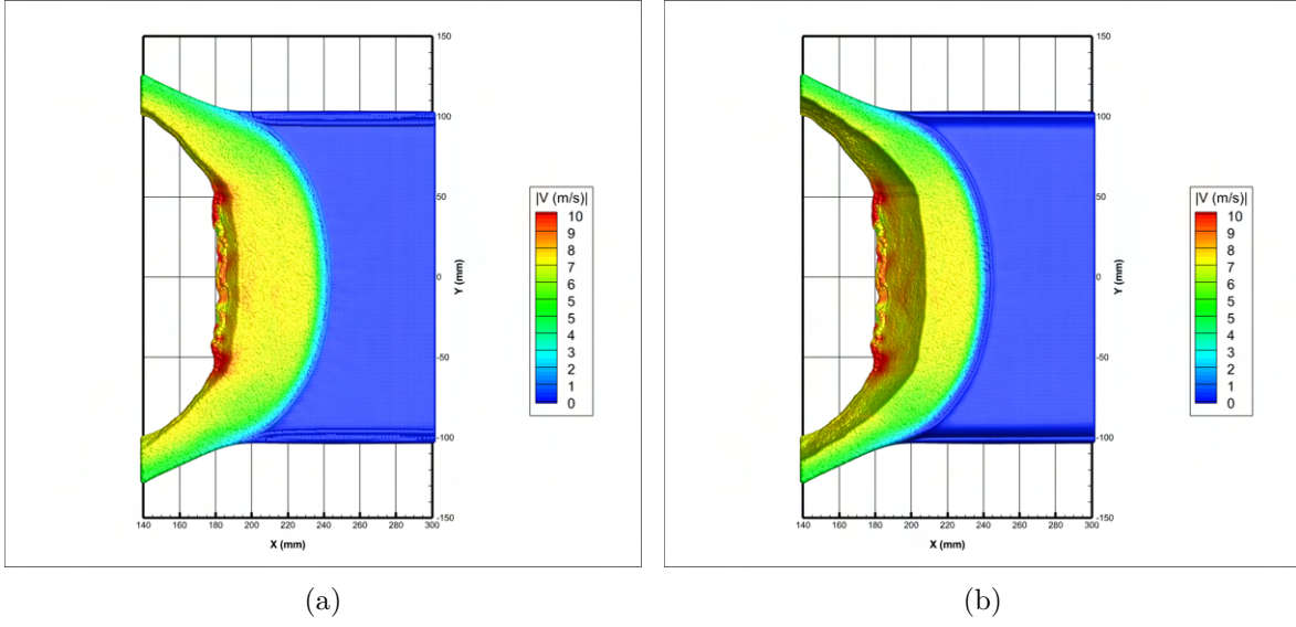
Figure 4.41 – (XY) view of the Slick225 ( H_w = 3mm ) at Z < 1mm (a) and Z < 3mm (b) from the numerical calculation. The colormap corresponds to the |\vec{V}| field. For clarity issues, only the fluid is represented (not the tire, nor the road), and also we limit the view between X = 140mm and X = 300mm .
