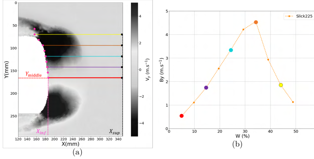
Figure 4.33 – In (a) we represent the positions of Y by the horizontal lines (only 1 position over 2 is represented for clarity reasons). To each of these positions correspond a value of B_y(W) plotted in (b). The same colors are used to designate the Y position and the corresponding B_y value. The X_{inf} and X_{sup} are highlighted successively with pink and black dots.
