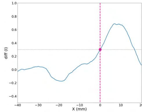
Figure 3.6 – \text{diff}(I) profile for the A6 worn at V_0=11.11\text{m.s}^{-1} and H_w = 1.5\text{mm} for \text{Img}_0 . The position of X_{\text{origin}} is highlighted with the vertical dashed line.
