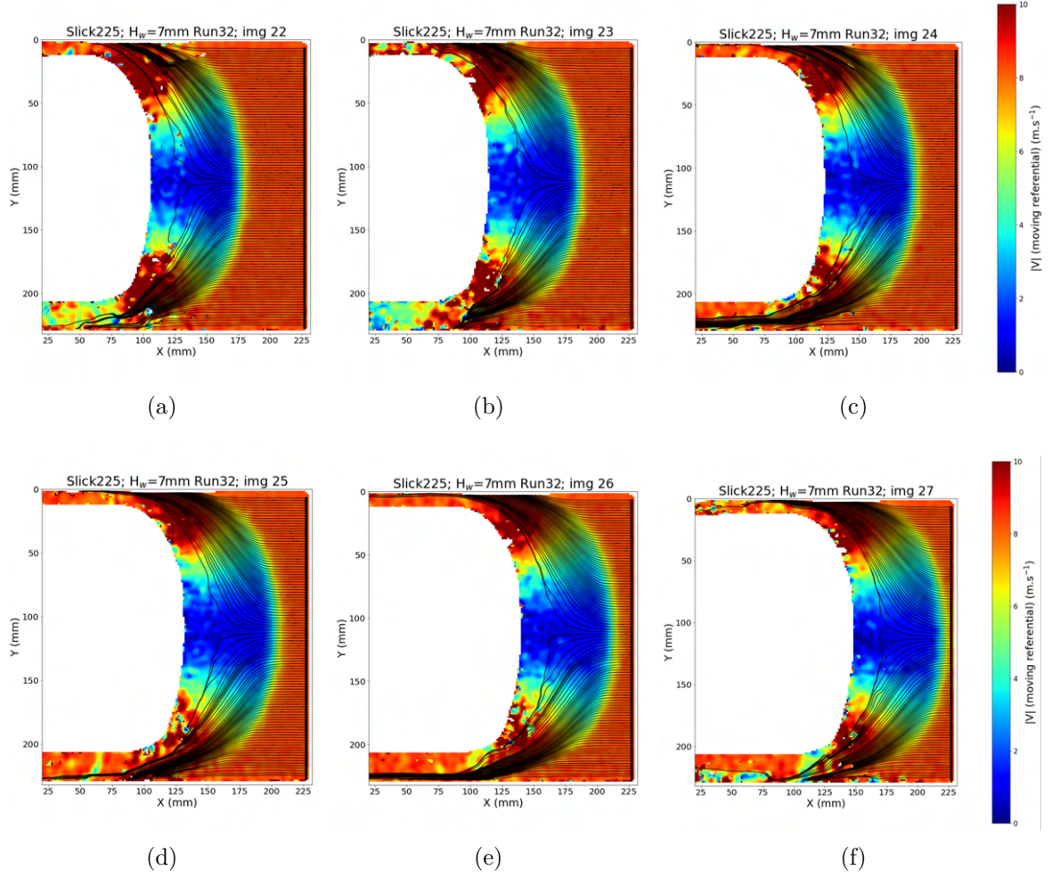
Figure 4.50 – Streamlines generation in the vehicle referential for the Slick225 at V_0 = 8.33 \text{ m.s}^{-1} and H_w = 7 \text{ mm} . The colormap corresponds to |V - V_0| . The instants t_{22} to t_{27} are depicted. The F0-F1 method is used.
