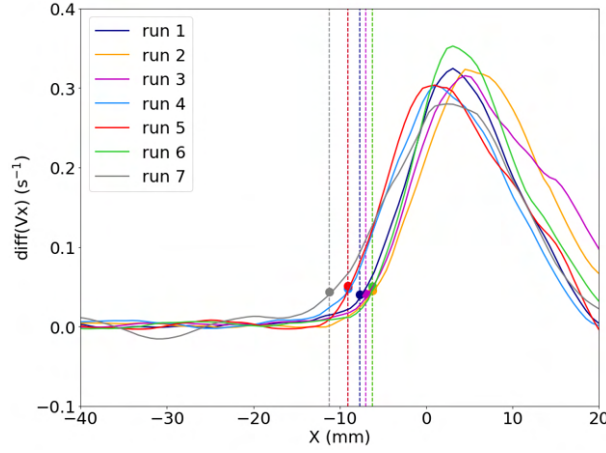
Figure 3.8 – \text{diff}(V_{jII}) profiles for the A6 worn at V_0=11.11\text{m.s}^{-1} and H_w = 1.5\text{mm} corresponding to the velocity profiles in Fig.3.7(d). The positions of X_{\text{slope } WB_j} are highlighted with the vertical dashed lines.
