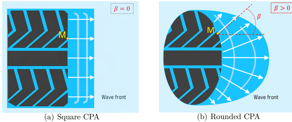
Figure 1.6 – Schematic representation of respectively a square (a) and a rounded (b) CPA with a highlight on the water drainage in front of the tire.
