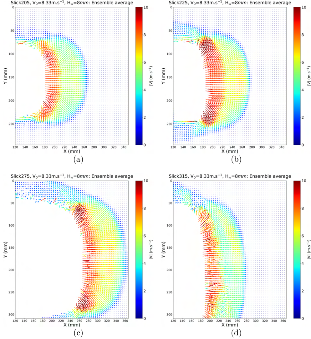
Figure 4.32 – Ensemble average velocity fields |\vec{V}| ( N = 8 ) for respectively the Slick205 (a), Slick225 (b), Slick275 (c) and Slick315 (d) at V_0 = 8.33 \text{ m.s}^{-1} and H_w = 8 \text{ mm} . For clarity reasons, only one arrow over 4 is represented.
