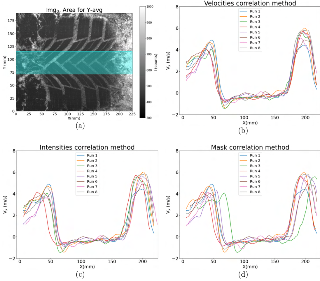
Figure 3.13 – Comparison between the three overlapping methods in the case of the A6 worn at V_0 = 8.33 \text{ m.s}^{-1} , H_w = 1.5 \text{ mm} and N = 8 runs. The V_x profiles of all runs are plotted Y-averaged in the area highlighted in blue in (a). Profiles obtained after using the correlation method are plotted in (b), after the intensities correlation in (c) and after the mask correlation in (d).
