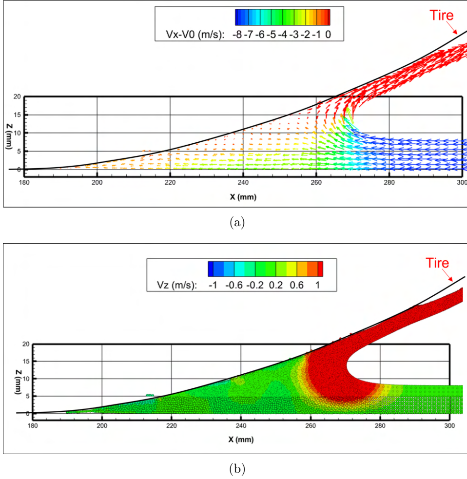
Figure 4.40 – XZ view in the middle of the WB between Y = -2.75\text{mm} and Y = 2.75\text{mm} . In (a) we represent the flow circulation with arrows in the vehicle referential, and in (b) we depict V_z . Case Slick225 H_w = 8\text{mm} .
