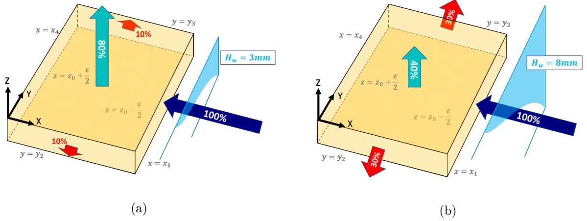
Figure 4.31 – Schematic representation of the mass fluxes in the WB when x_4 is close to the tire for H_w = 3mm (left) and H_w = 8mm (right)
