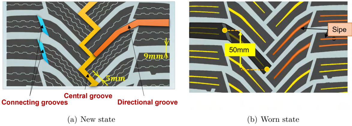
Figure 6.5 – Details of the A6 tread design at new (a) and worn (b) state respectively.
