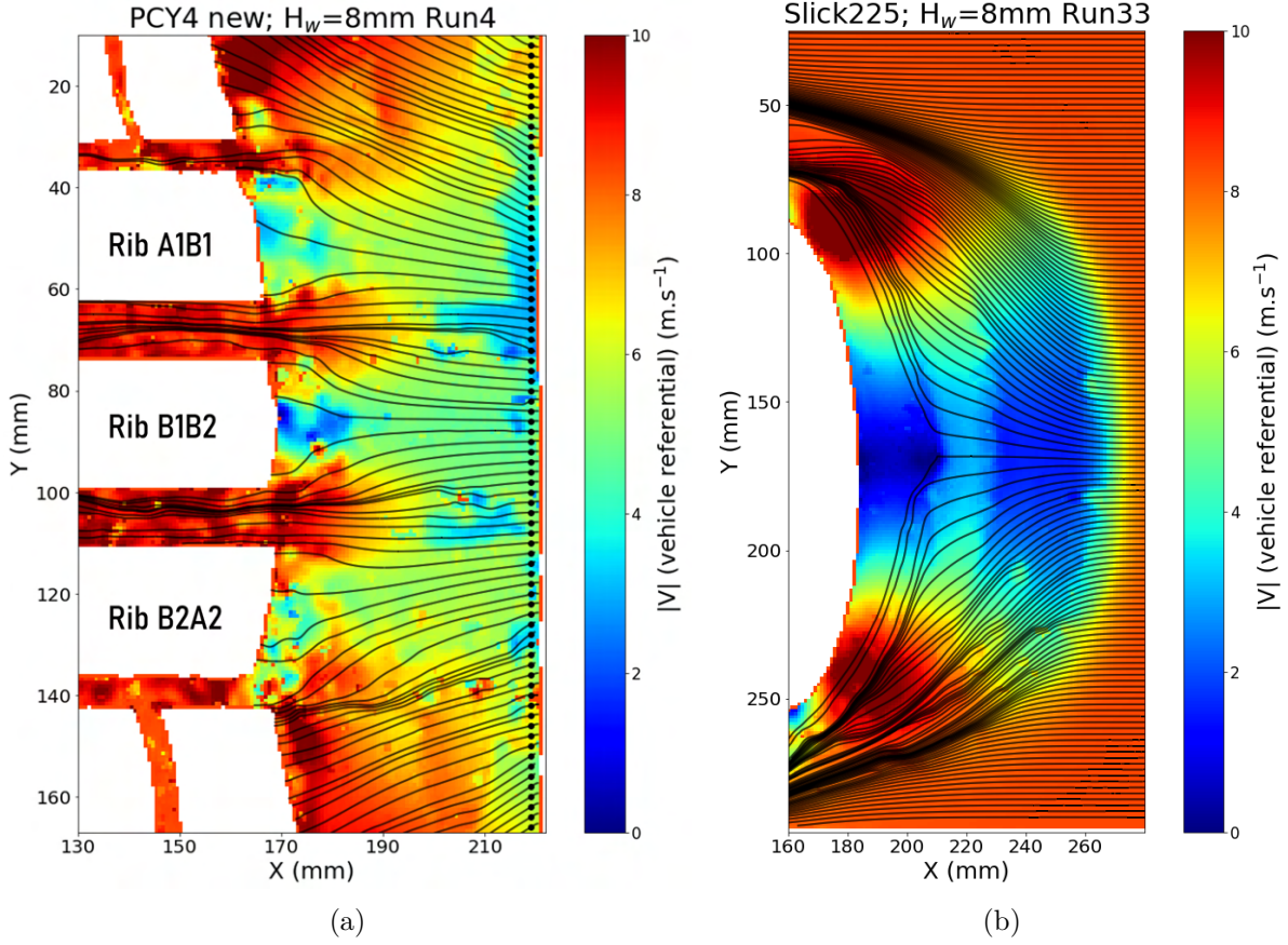
Figure 5.16 – Streamlines generation for the PCY4 new (a) and Slick225 (b) along with the |\vec{V}| field: r-PIV measurements at V_0 = 8.33 \text{ m.s}^{-1} and H_w = 8 \text{ mm} .
