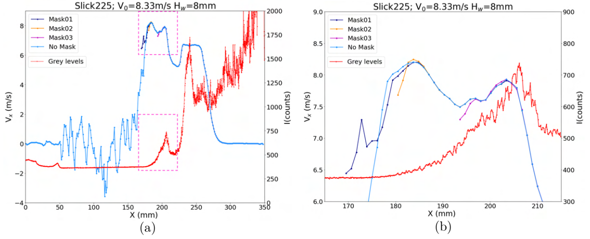
Figure 4.5 – Grey-level image intensity and velocity profiles Y-averaged in the area of interest (delimited by the two blue horizontal lines in Fig.4.3 (a)) of the configurations with masks and the one without a mask. The same profiles are represented in (b) but zoomed in the area outlined with the pink dotted rectangles in (a) (corresponding to the Y-averaged velocity inside the blue rectangle in Fig.4.3 (a)).
