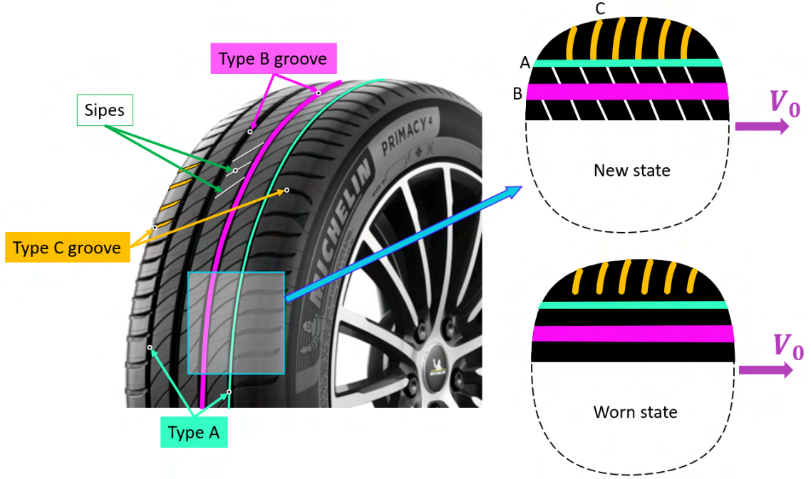
Figure 5.1 – Details of the PCY4 tread design with highlights of the different groove types: A (green), B (pink), C (orange), and sipes (white). On the right is a simplified sketch of the CPA for both new (upper part) and worn (lower part) states. Since the tread is symmetric, only the upper half of the CPA is sketched for simplification issues.
