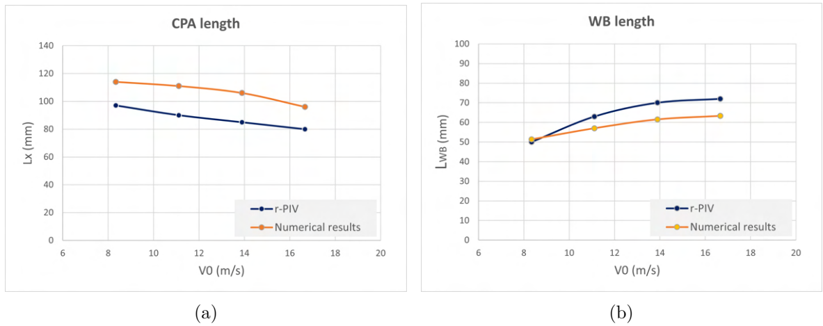
Figure 5.15 – Contact patch length (a) and water-bank length (b) evolution for different V_0 values obtained both experimentally and numerically.
