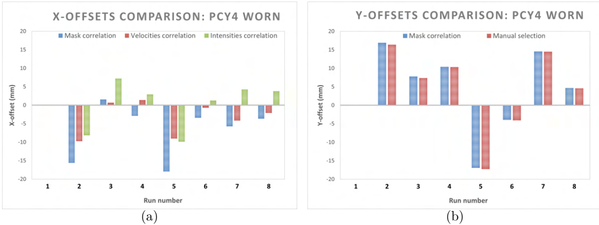
Figure 3.10 – X-offsets (a) and Y-offsets (b) generated using the different offsetting strategies in the case of the PCY4 worn at V_0 = 8.33m.s^{-1} , H_w = 1.5mm and N = 8 runs.
