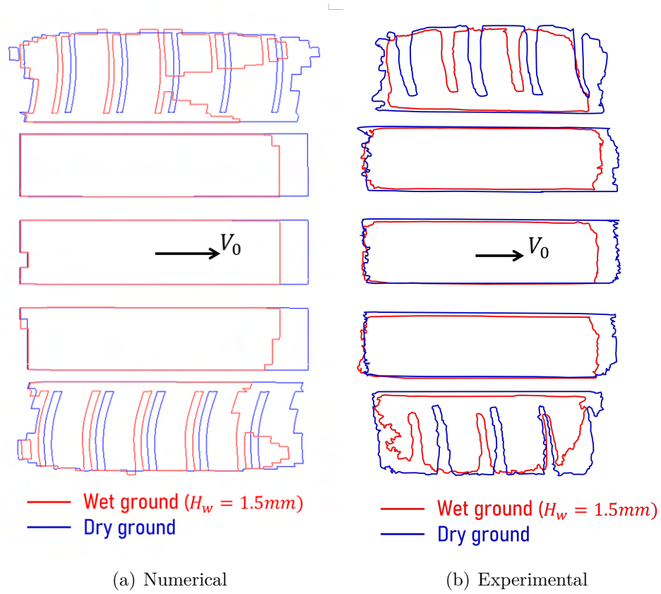
Figure 5.6 – PCY4 at V_0 = 13.89m.s^{-1} , H_w = 1.5mm .
