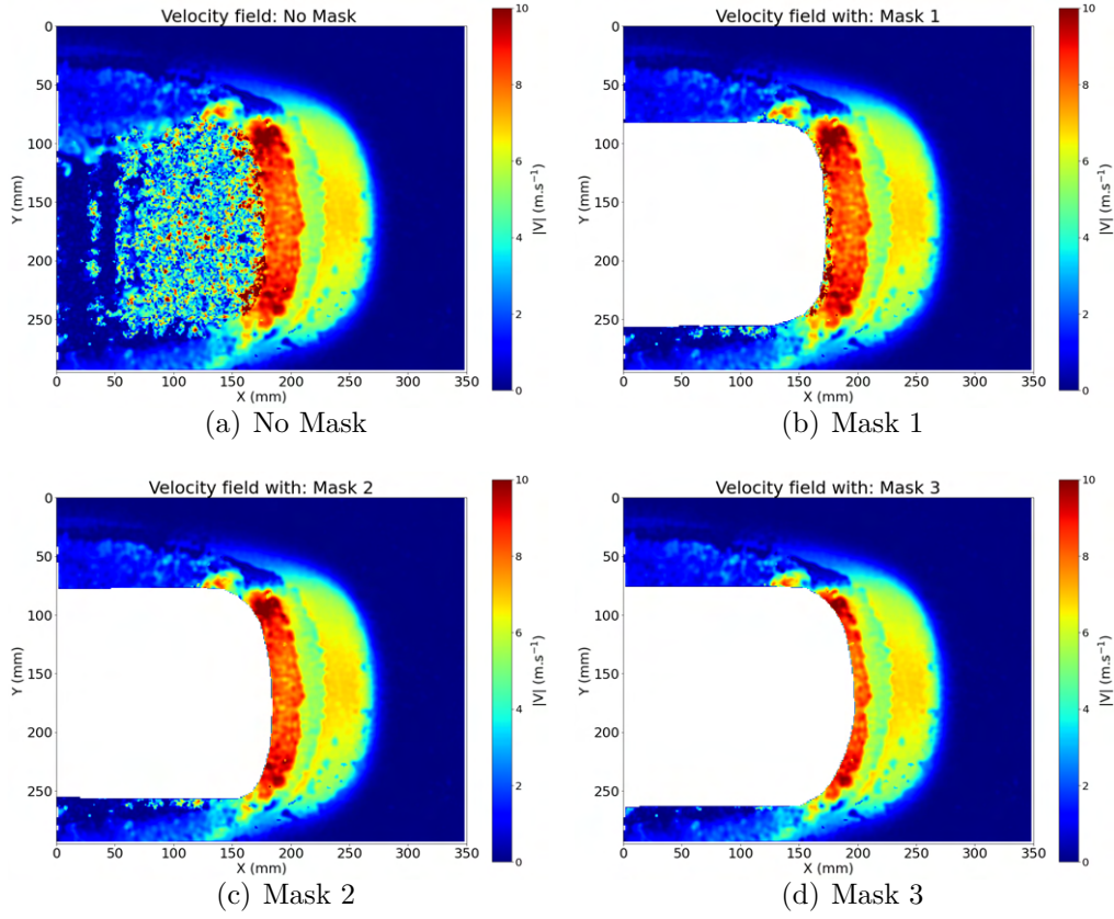
Figure 4.4 – Velocity field |\vec{V}| for the Slick225 at V_0 = 8.33 m.s^{-1} and H_w = 8 mm , (a) without applying a mask, and respectively after applying Mask01 (b), Mask02 (c) and Mask03 (d). The cross-correlation parameters used are of the REF case in Table 4.1.
