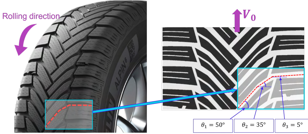
Figure 6.1 – Details of the Alpin 6 tread design with a highlight on a unique directional groove and its directions with respect to the horizontal axis.
