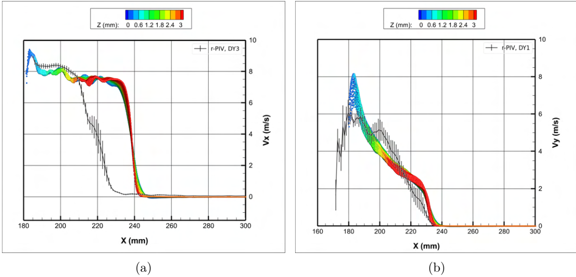
Figure 4.42 – Evolution of V_x with X between Y = -2.75mm and Y = 2.75mm (a), and V_y with X between Y = 47.5mm and Y = 52.5mm (b). The colors represent the altitude Z of the particle, and each point represents an SPH particle. We overlay the corresponding r-PIV results with the error bars representing the standard deviation between the N runs. Case Slick225 H_w = 3mm .
