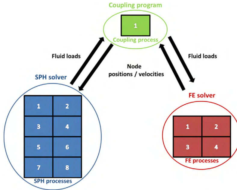
Figure 2.6 – Example of an SPH-FE coupling strategy where 8 cores and 4 cores respectively for SPH and FE solvers are used, and a single core is dedicated to the coupling program (Hermange et al. [48]).
