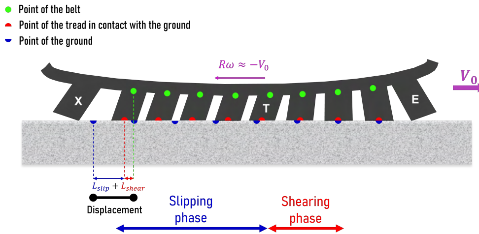
Figure 1.4 – Contact between tire blocks and dry ground during the braking phase. The tire is moving to the right ( V_0 ), and the tire rotation is indicated with the R\omega \approx -V_0 arrow. The tread block E is entering the contact region while block X is leaving it. Starting from block T, the blocks are slipping since the maximum shearing is reached.
