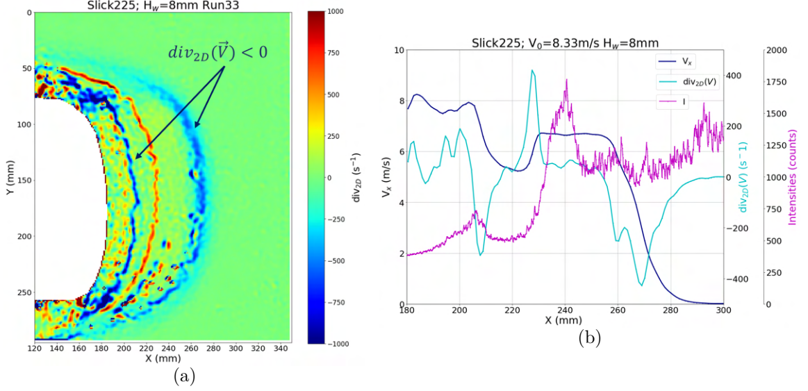
Figure 4.13 – Cartography of the 2D divergence of the velocity ( div_{2D}(\vec{V}) ) (left) and the V_x , div_{2D}(\vec{V}) and intensity profiles Y-averaged between Y = 140\text{mm} and Y = 195\text{mm} (right): Run33
