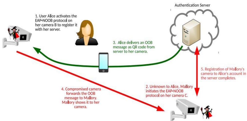
Figure 11: IoT Threat Attack Scenario [112]
