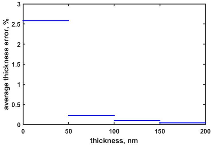
Figure 6-1 Average thickness error measured with the Broadband monitoring setup.
