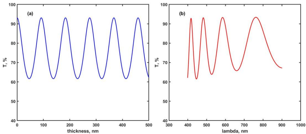
Figure 1-4. (a) - Transmittance evolution depending on the layers thickness, (b) - transmittance spectra of 500 nm thick Nb_2O_5 layer.
