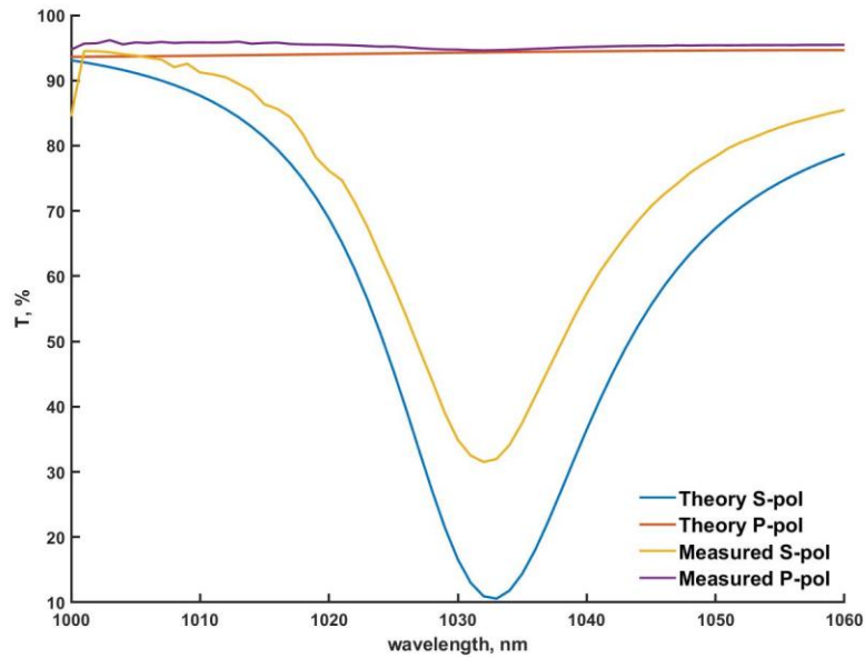
Figure A5-1 Measured and theoretical performance of the D5D3 component
