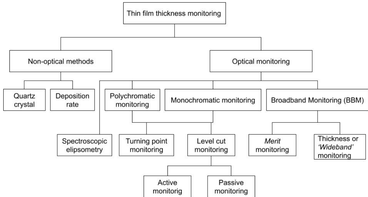
Figure 2-5 Schematic overview of the monitoring methods.
