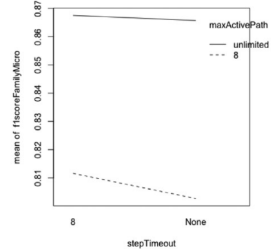
(i) Step timeout and max active path
