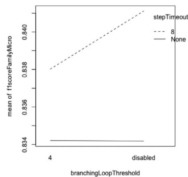
(h) Branching loop and step timeout
