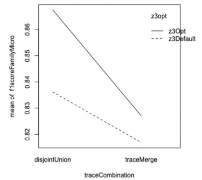
(c) Trace combination and z3 configuration
