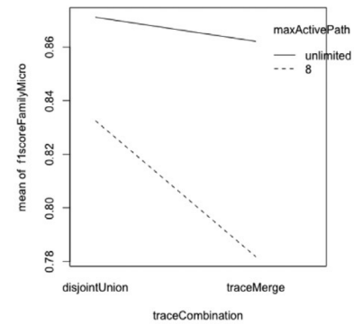
(f) Trace combination and max active paths
