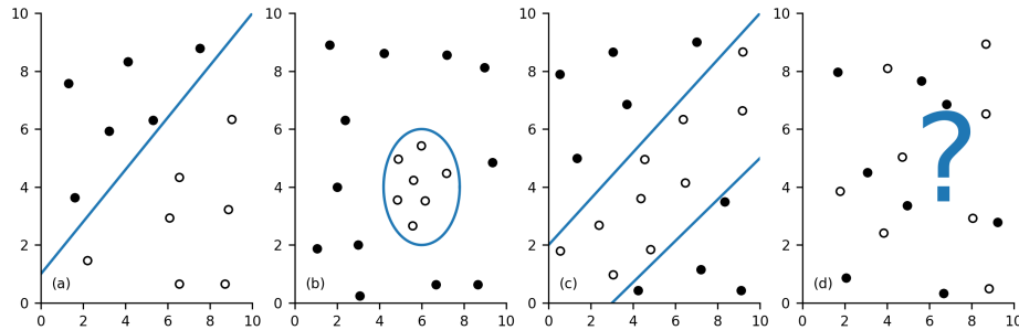
Figure 2.2: Single layer artificial neural networks such as the perceptron can only classify linearly separable data. (a) is linearly separable. (b) is not linearly separable. However, data are contained in an ellipse. The equation of an ellipse is of the form a \times x^2 + b \times y^2 = 1 , so if we transform the feature variables into X = x^2 and Y = y^2 , the data become linearly separable. (c) is equivalent to a fundamental XOR gate, and is not linearly separable, which was part of the reasons for the first AI winter. It can either be solved by combining several layers of artificial neurons, or by complex kernel tricks which map the data from the original space into a higher dimensional space where they become linearly separable. (d) is possibly not separable at all. AI: Artificial Intelligence. XOR: Exclusive OR.
