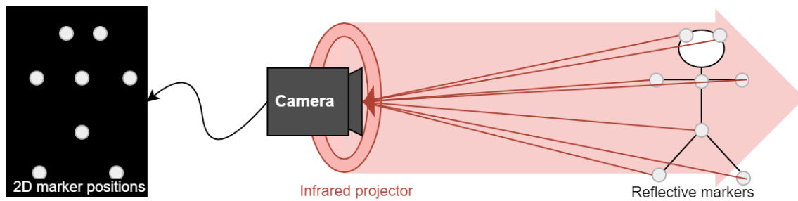
(a) An opto-electronic camera is traditionally surrounded by a crown of infrared LEDs, projecting light toward the subject. The subject wears markers, which reflect light back to the camera. Marker positions are then known in the camera plane.
