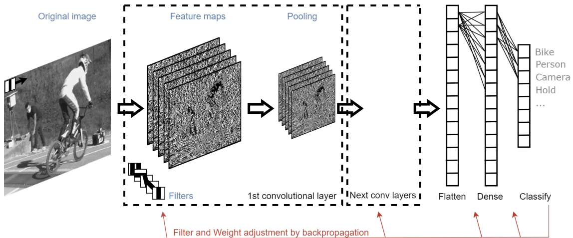
Figure 2.5: A simplified convolutional neural network (CNN.) A convolutional layer consists of a series of filters running across the input image, and producing feature maps, which are then downsampled by pooling. Filters become more and more elaborated along layers, and produce feature maps which look like whole object parts. Filters and weights are randomly initialized at first, and then are adjusted by backpropagation. After the convolutional layers, the feature maps are flattened to produce a 1D vector, which is then processed by dense layers, and finally a softmax layer computes a probability for the image to correspond to each available class.
