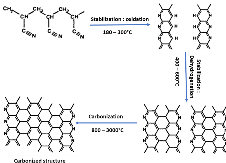
Figure 2.3 Illustration of some steps of the process of converting PAN fiber into carbonized structure. Modified from [2]
