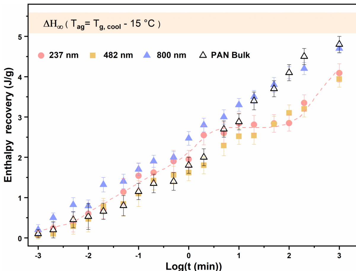
Figure 3.11 Enthalpy recovery as a function of aging times of PAN nanofibers with the average diameters 237nm (orange circles) 482 nm (yellow squares) 800 nm (blue triangles) bulk PAN (empty triangles), the pink dashed line is to guide the eye
