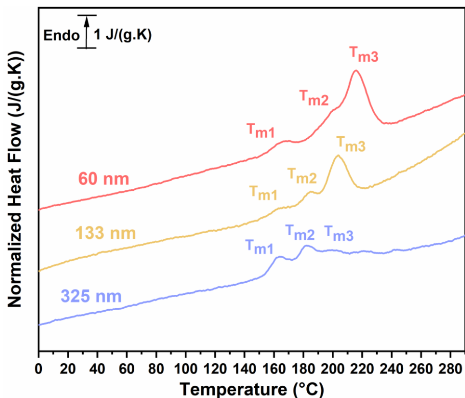
Figure 4.11 FSC heating scans of PA6 nanofiber mats with different nanofiber diameters normalized to the sample mass and the heating rate 120\ 000\ \text{K}\cdot\text{min}^{-1}
