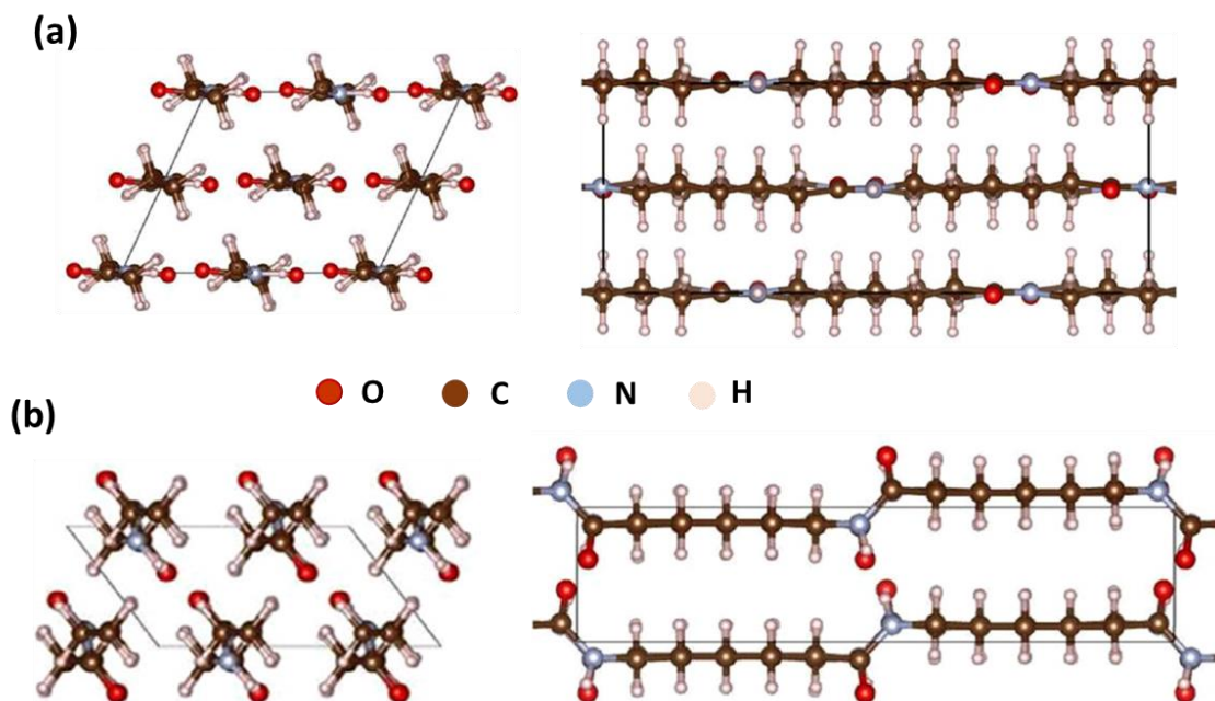
Figure 4.3 Schematic illustration of the atomic configuration of polyamide 6 (a) \alpha and (b) \gamma crystalline forms [51]
