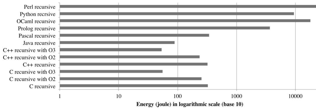
Figure 4.2: Energy consumption of a recursive implementation of Tower of Hanoi program in different languages [102].
