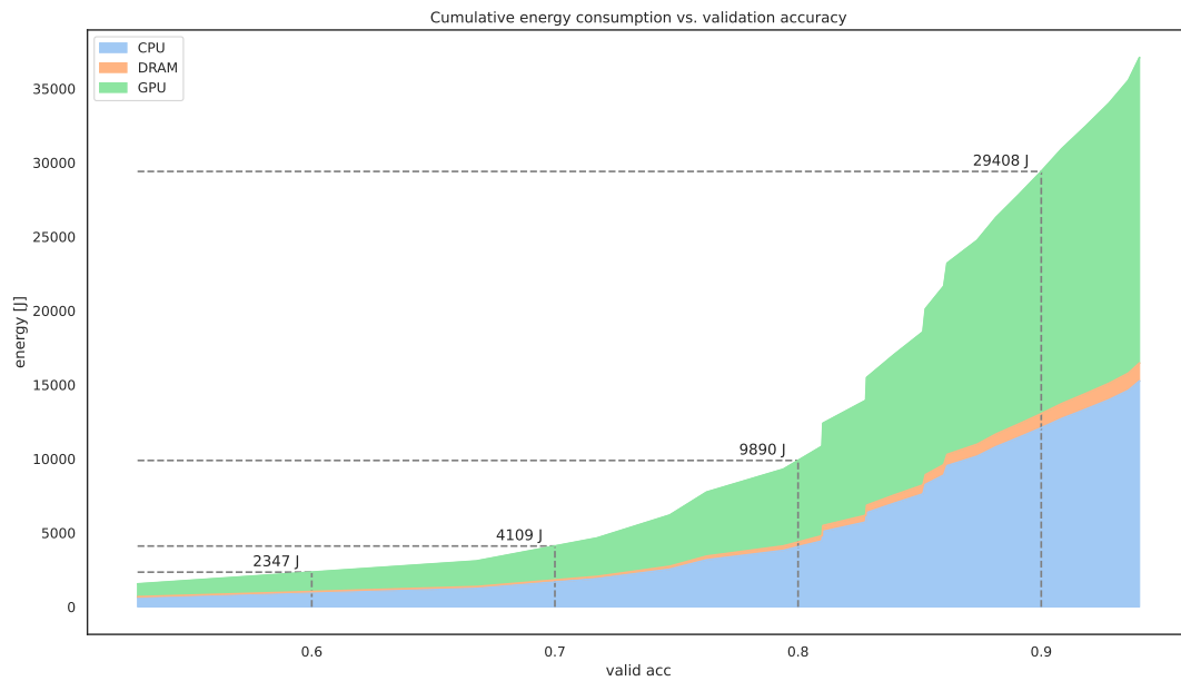
Figure 4.5: Cumulative energy consumption vs. accuracy [74].
