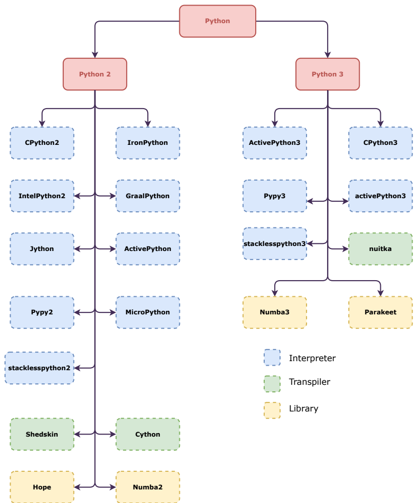
Figure 4.16: Python interpreters
