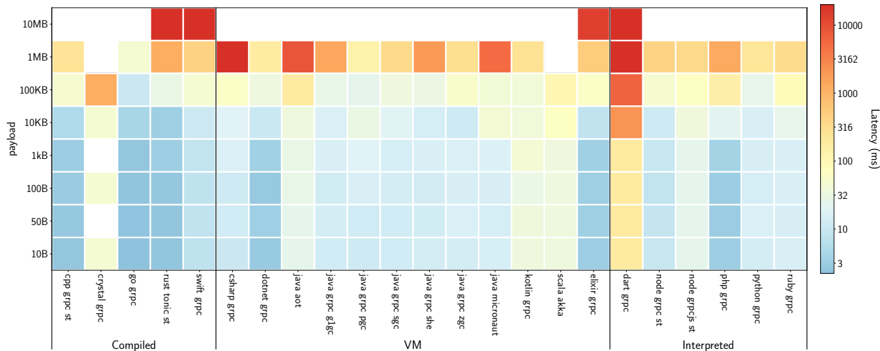
Figure 6.7: Tail latency (99%) based on the request size
