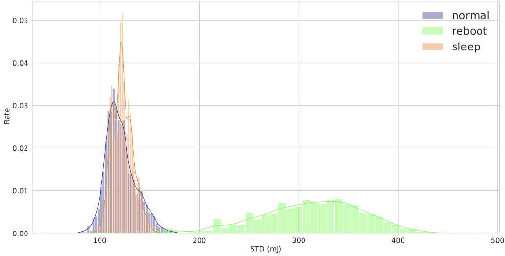
Figure 3.8: STD analysis of the normal, sleep and reboot modes
