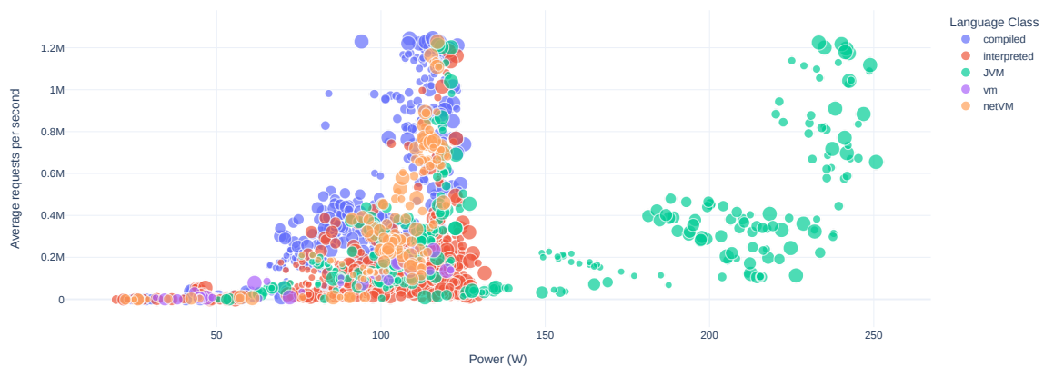
Figure 6.23: total request vs. average power consumption for JSON Serialization scenario (size of circles represents the number of clients)
