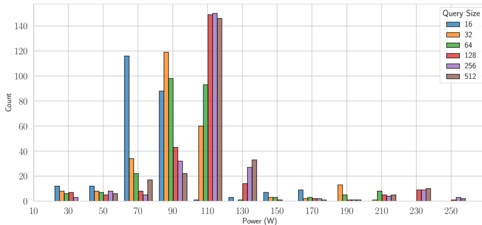
Figure 6.15: Distribution of the average power consumption for single query scenario
