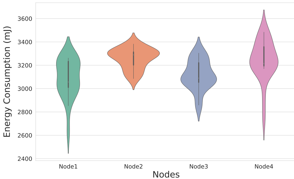
Figure 2.4: CPU energy variation for the benchmark CG
