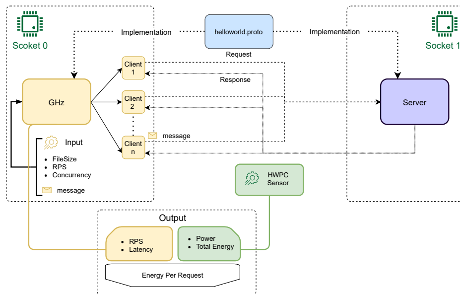
Figure 6.1: Experimental software architecture.
