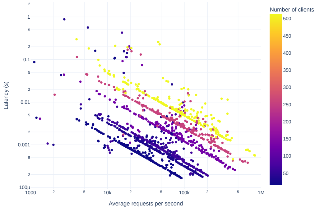
Figure 6.12: Correlation of latency and number of requests per second for a single query
