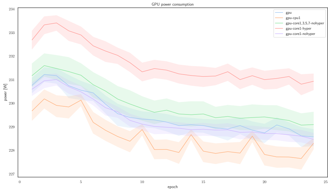
Figure 4.7: Evolution of average GPU power along epochs [73].
