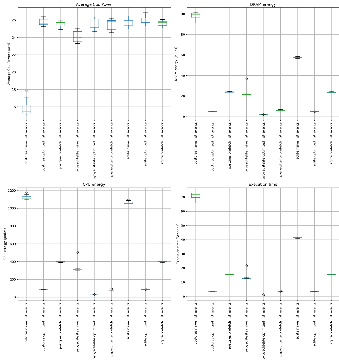
Figure 4.11: Key performance indicators observed for different data access strategies.
