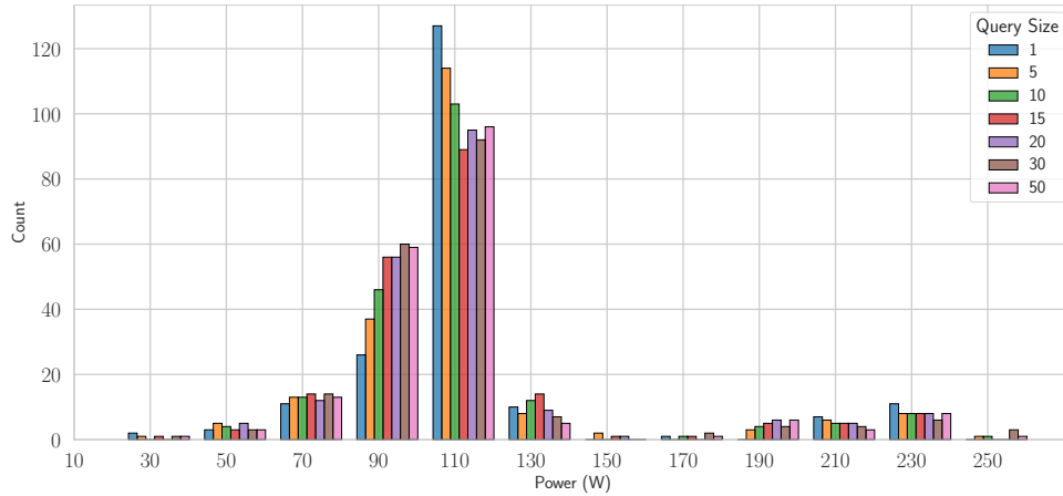
Figure 6.17: Distribution of average power consumption for the multiple queries scenario
