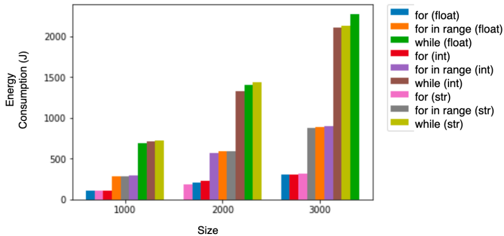
Figure 4.13: Comparison of the energy consumption of different Python loops [125].
