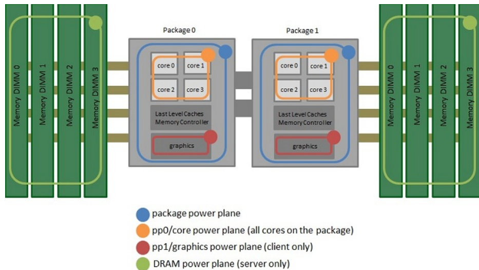
Figure 2.3: INTEL RAPL scopes
