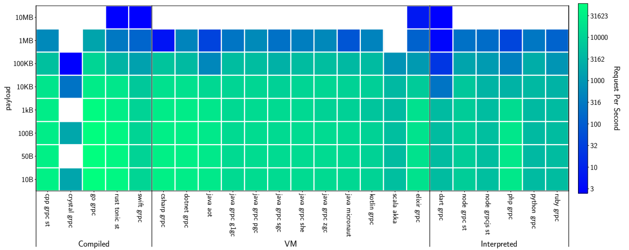
Figure 6.8: Number of requests per second based on the request size
