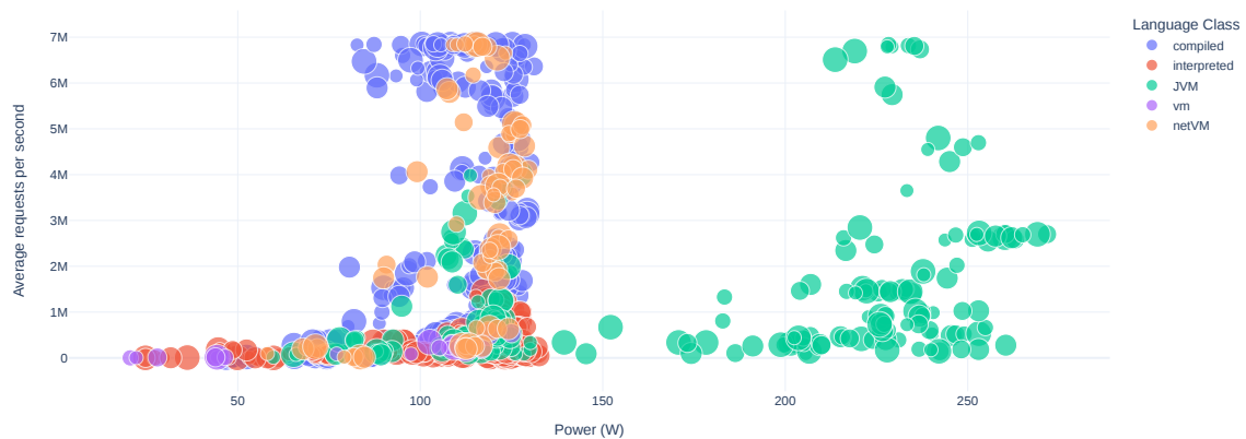
Figure 6.22: Total request vs. average power consumption for plainText scenario (size of circles represents the number of clients)
