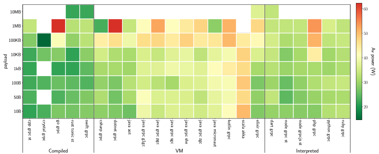
Figure 6.6: Average power consumption based on the request size
