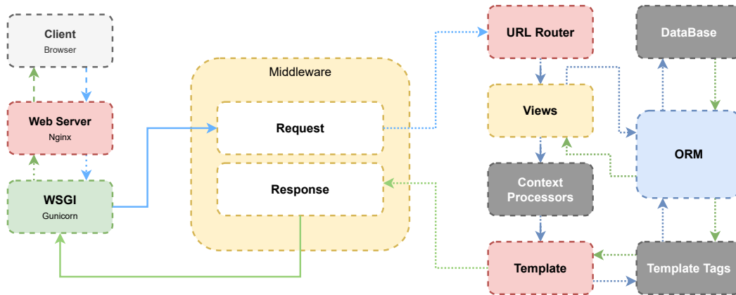
Figure 4.9: Request-Response life cycle in Django
