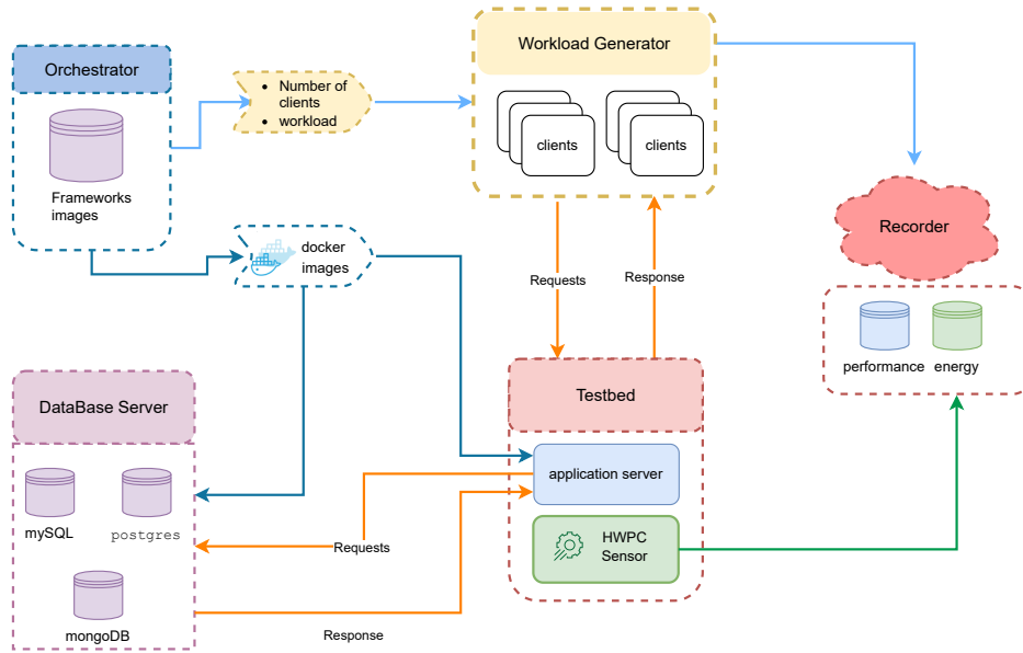
Figure 6.10: Architecture of the experiments.
