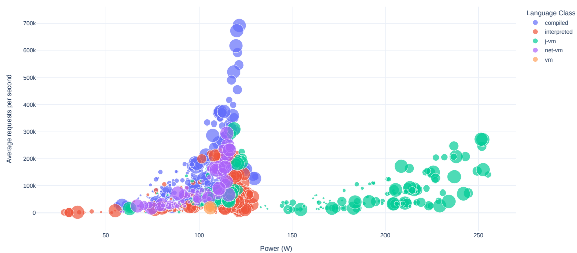
Figure 6.21: Total request vs. average power consumption for Fortunes scenario (size of circles represents the number of clients)
