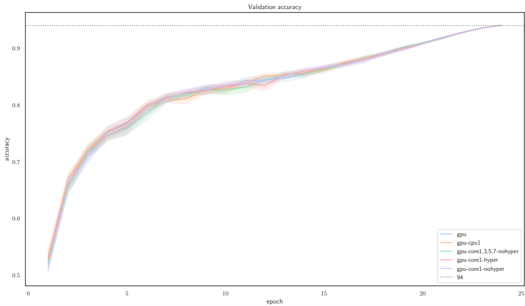
Figure 4.4: Accuracy along epochs [73].
