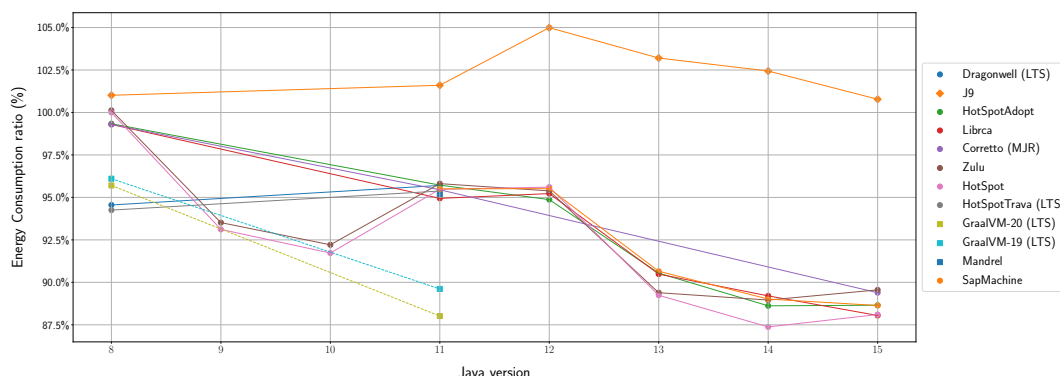
Figure 5.3: Energy consumption evolution of selected JVM distributions along versions.
