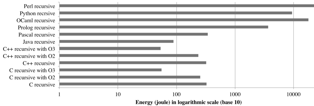
Figure 4.2: Energy consumption of a recursive implementation of Tower of Hanoi program in different languages [101].
