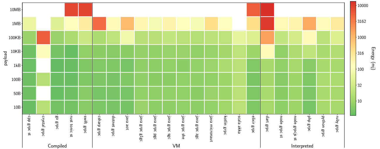
Figure 6.9: Energy consumption based on the request size
