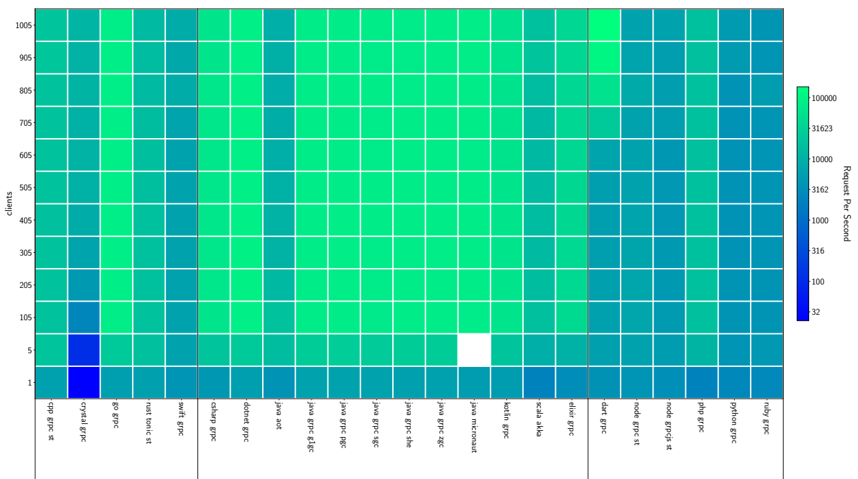
Figure 6.3: Number of requests per second based on the number of clients
