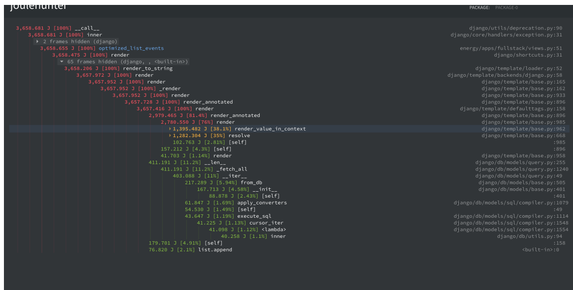
Figure 4.12: Tree representation of the energy consumption of a request in Django (optimized version)
