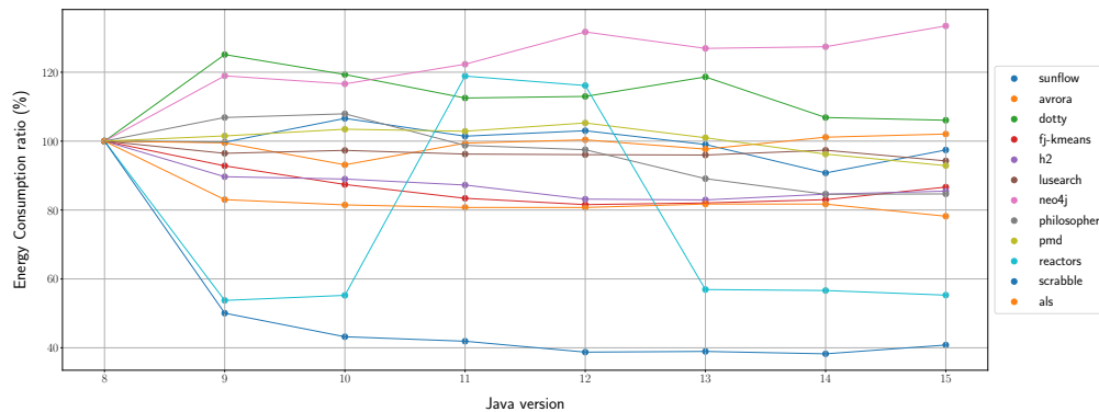
Figure 5.4: Energy consumption of the HotSpot JVM along versions.
