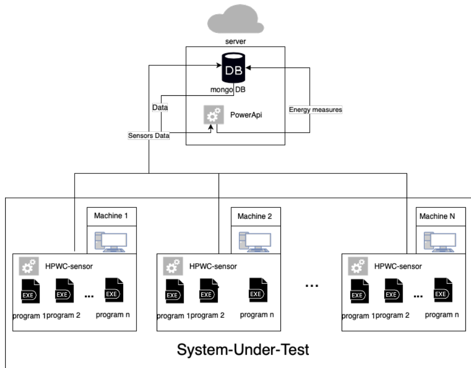
Figure 4.17: Benchmarking architecture deployed with POWERAPI.
