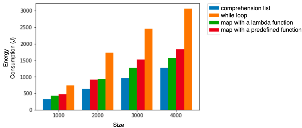
Figure 4.14: Comparison of the energy consumption of different methods to convert a list [125].
