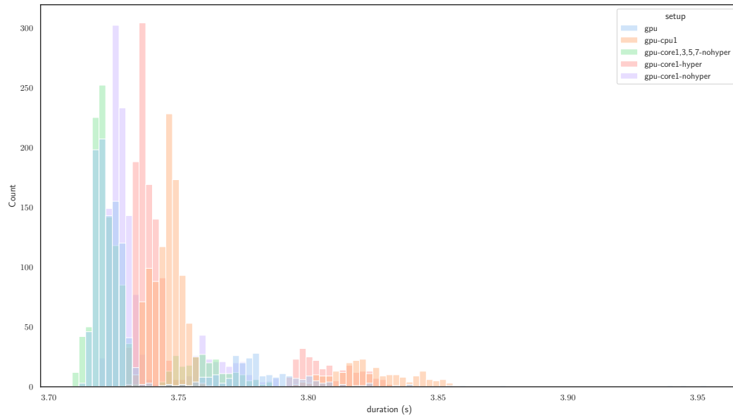
Figure 4.8: Distribution of the durations of each epoch [73].
