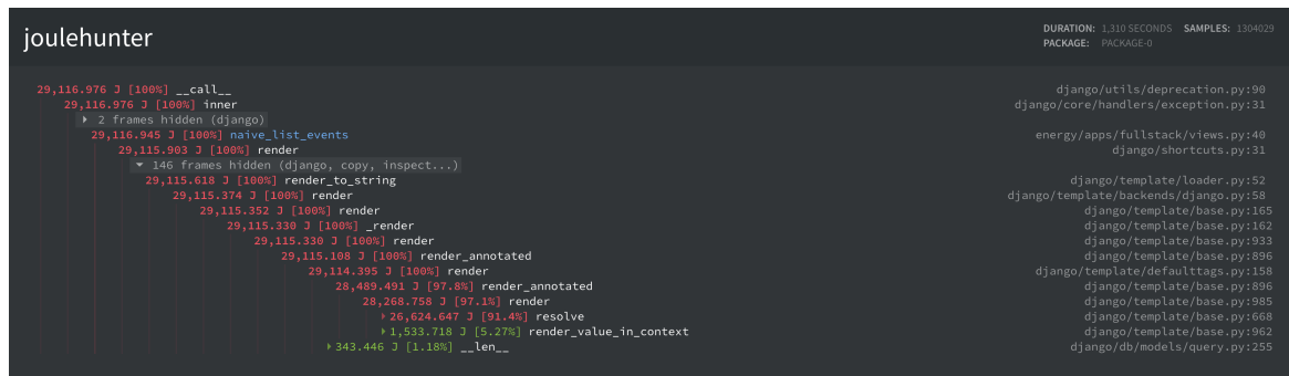
Figure 4.10: Tree representation of the energy consumption of a single request in Django (naive version).
