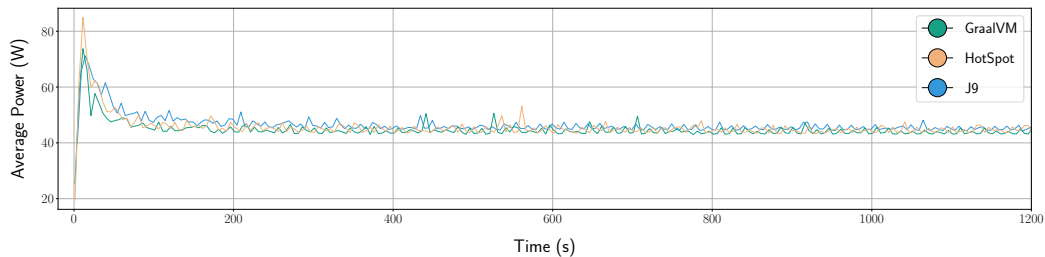
Figure 5.7: Power consumption of Dotty as a service for HOTSPOT, GRAALVM & J9.
