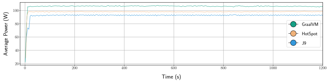
Figure 5.6: Power consumption of Scrabble as a service for HOTSPOT, GRAALVM & J9.
