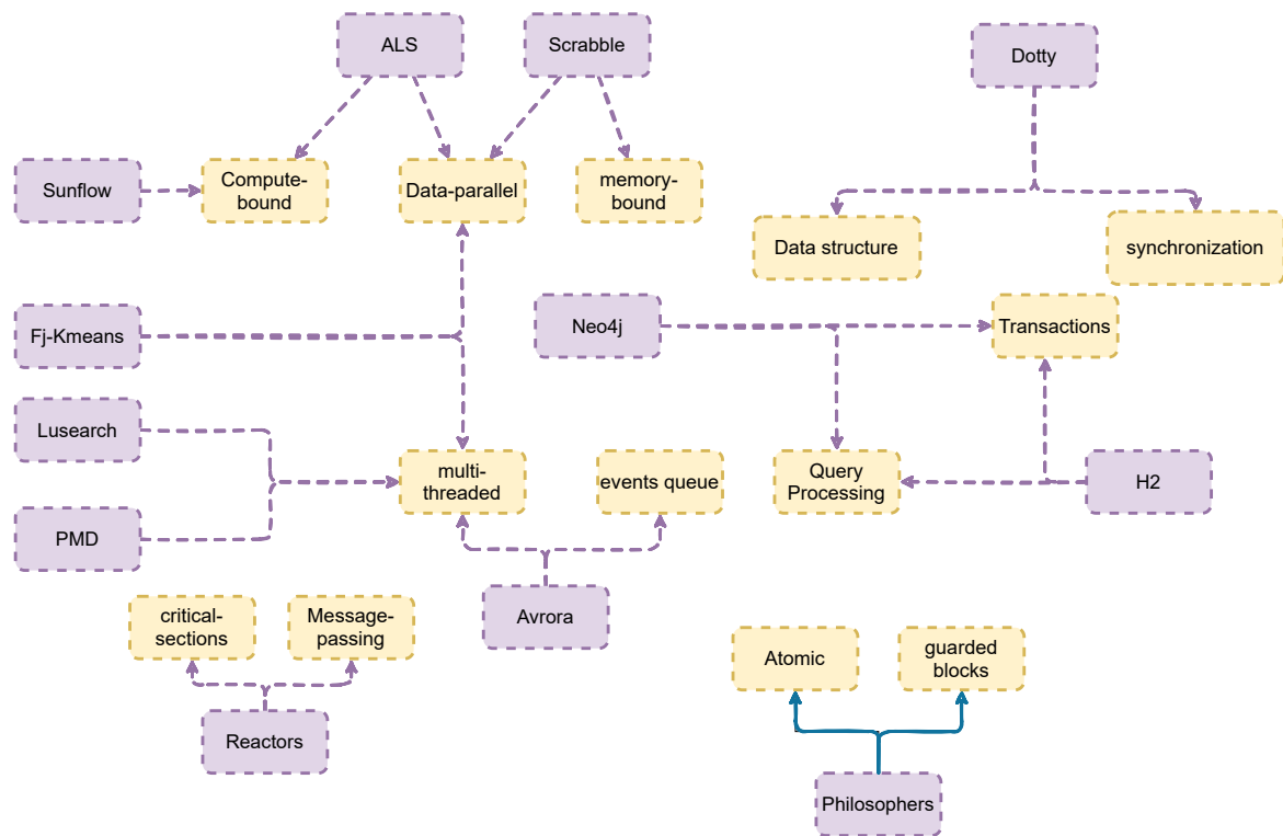
Figure 5.2: Target scope of DCAPO and RENAISSANCE benchmarks.
