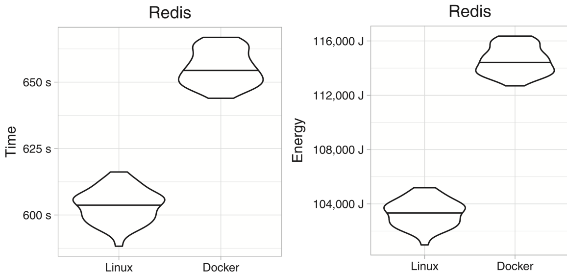
Figure 3.3: Execution time & energy consumption of Redis with and without Docker [41]
