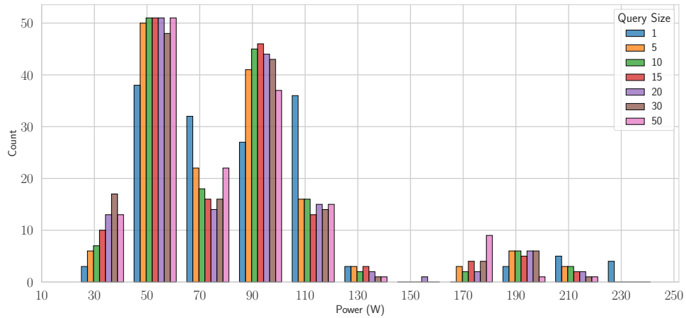
Figure 6.19: Distribution of the average power consumption for the update scenario
