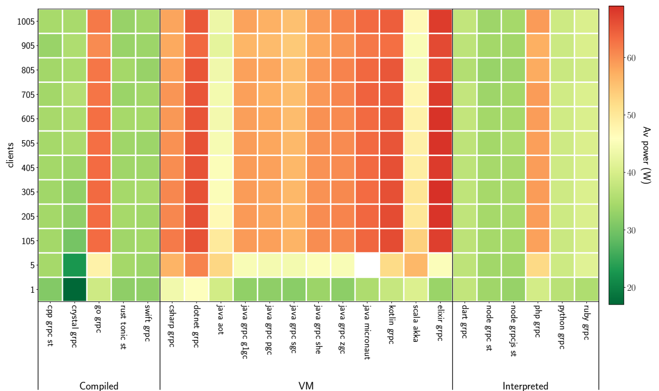
Figure 6.2: Average power consumption based on the number of the clients
