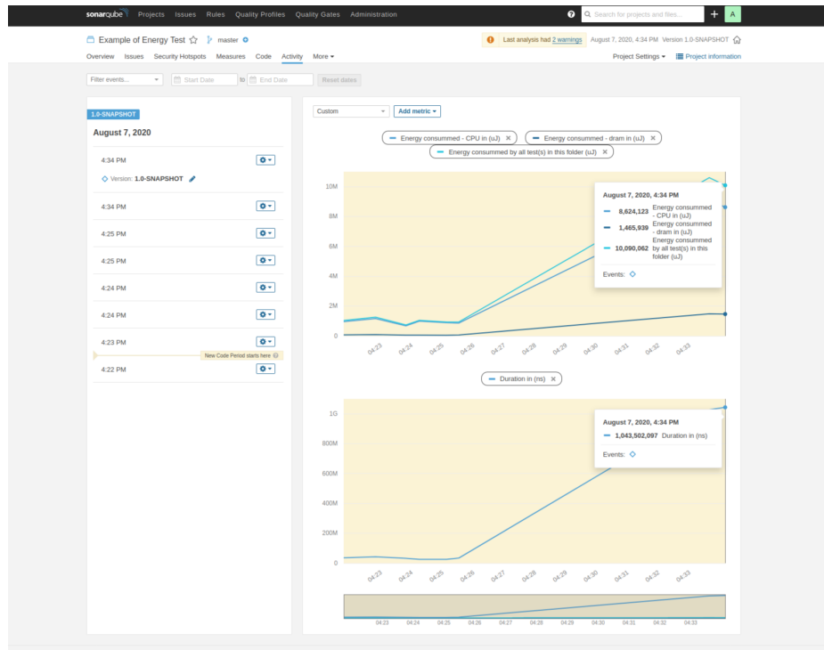
Figure 7.1: Sonar Energy plugin for JUnit
