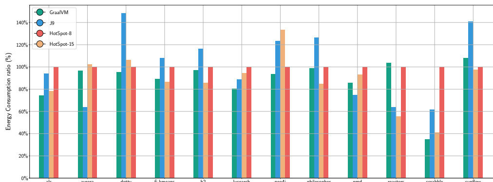
Figure 5.5: Energy consumption comparison across Java benchmarks for HOTSPOT, GRAALVM & J9.
