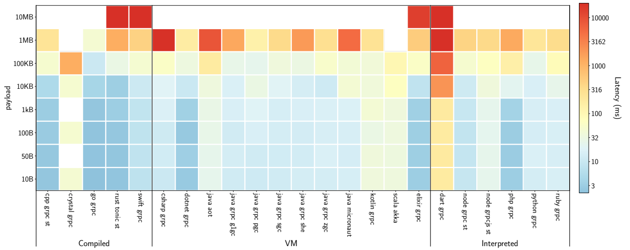
Figure 6.7: Tail latency (99%) based on the request size
