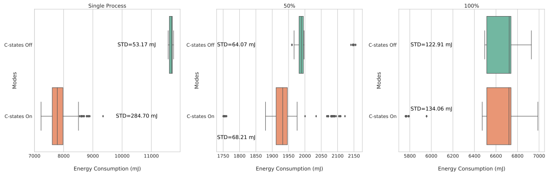
Figure 3.9: Energy variation when disabling the C-states
