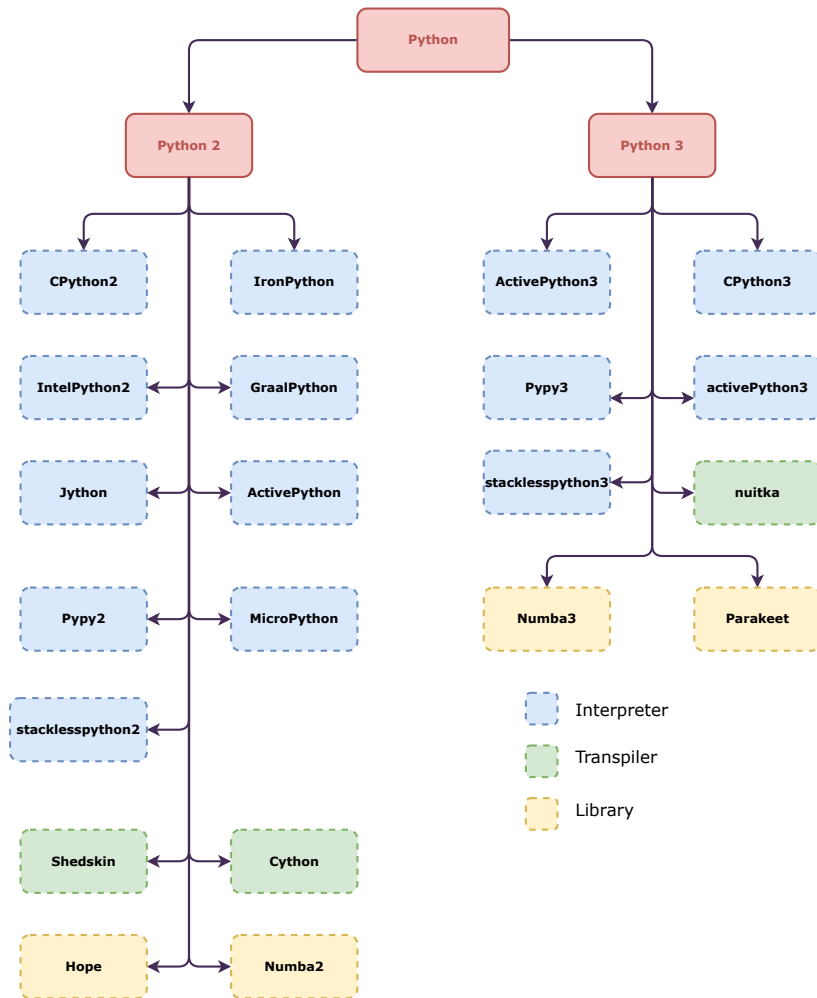
Figure 4.16: Python interpreters
