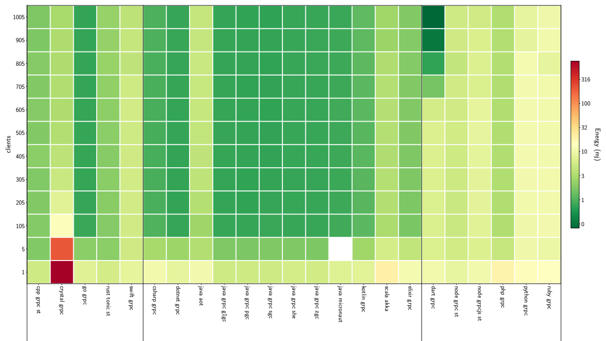
Figure 6.5: The cost of a single request based on the number of clients (mJ)
