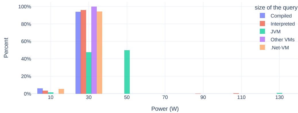
Figure 6.13: Average power consumption for the idle scenario
