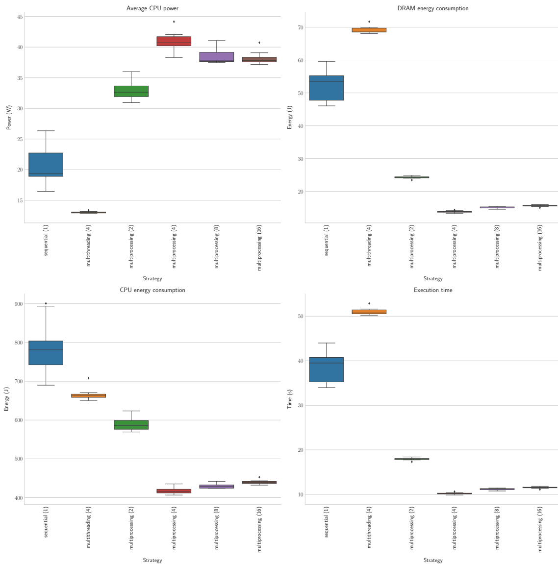
Figure 4.15: Energy consumption resulting from different Python concurrency strategies (number of workers).
