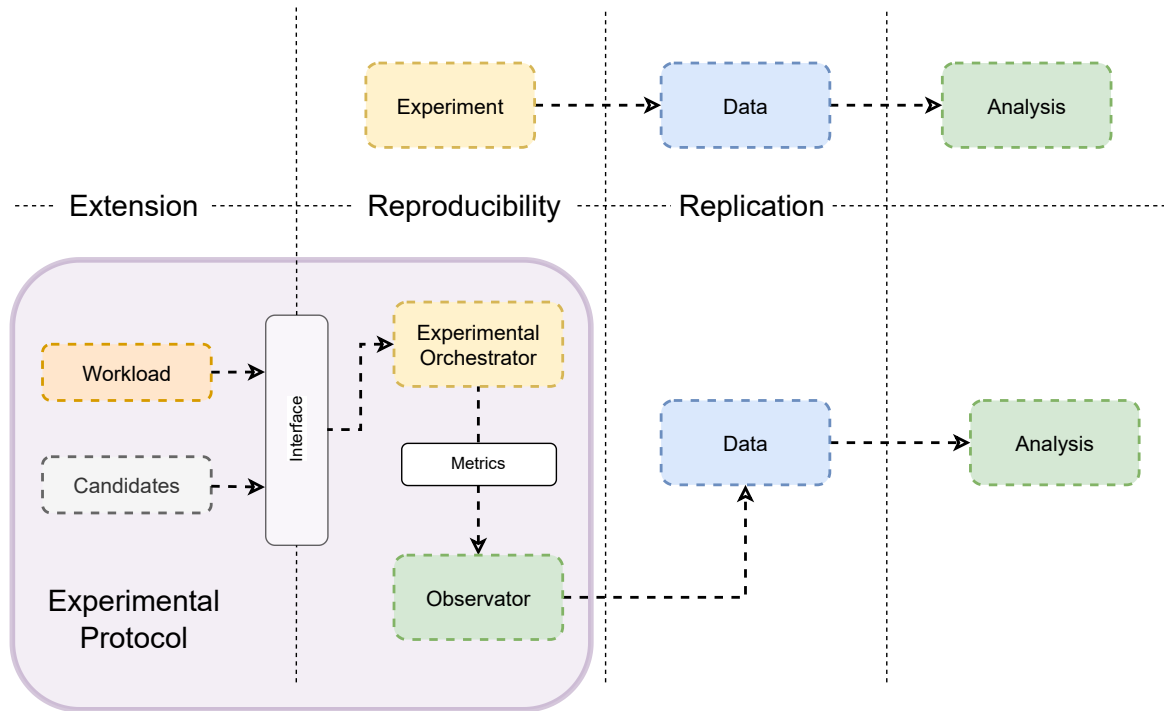
Figure 3.4: Benchmarking protocol
