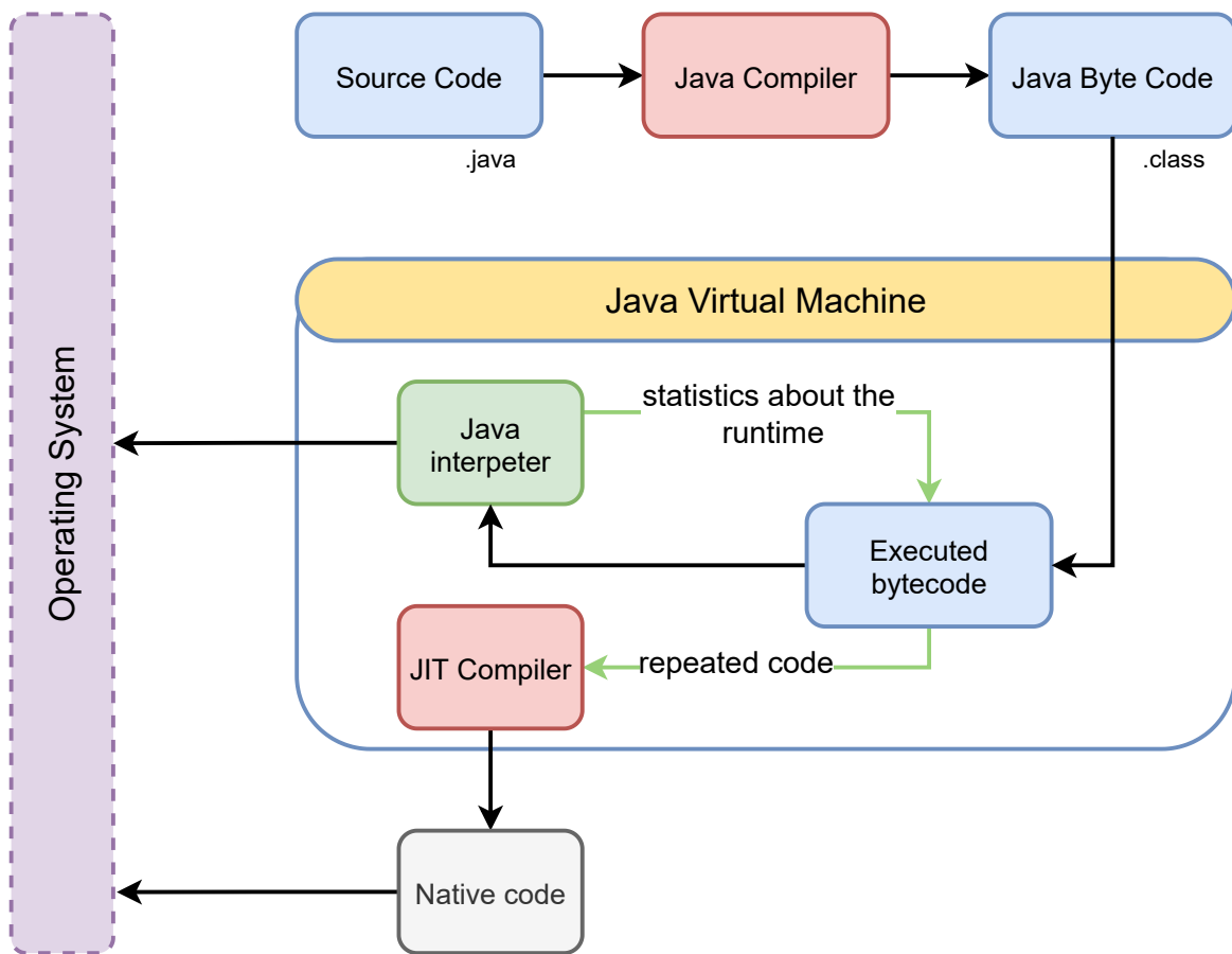
Figure 5.1: JVM architecture
