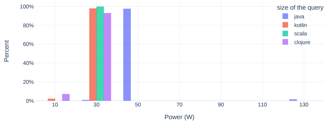
Figure 6.14: Average power consumption for Java-based languages in the idle scenario case
