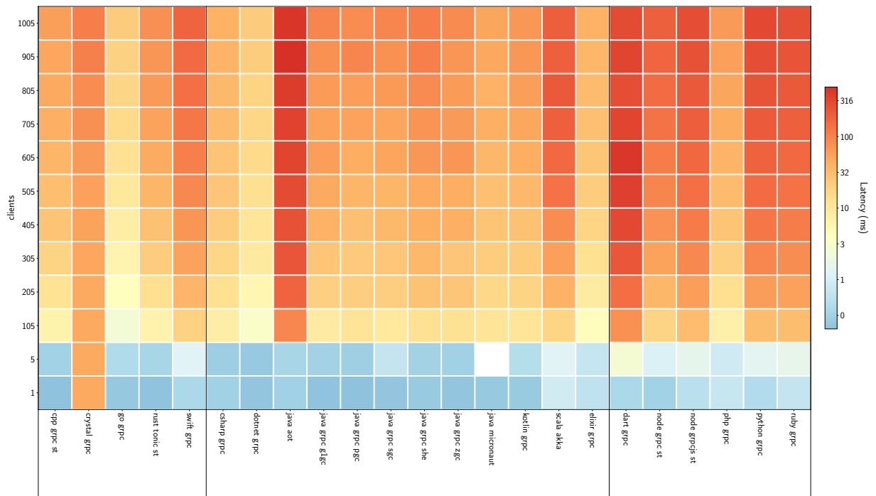
Figure 6.4: Tail latency (99%) based on the number of clients
