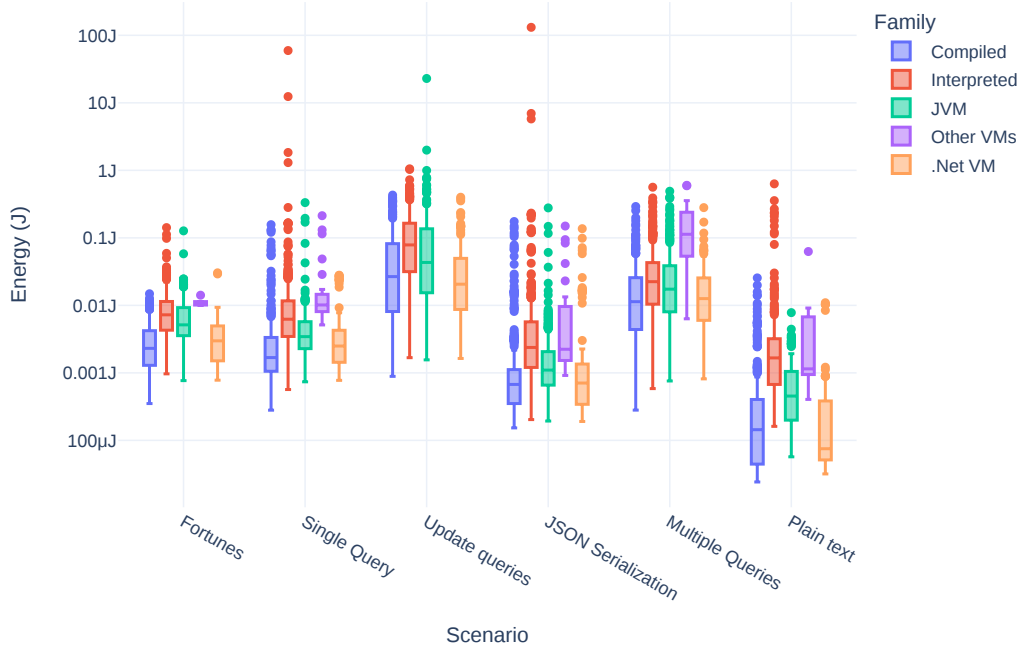
Figure 6.25: Energy consumption per request for each family of programming languages
