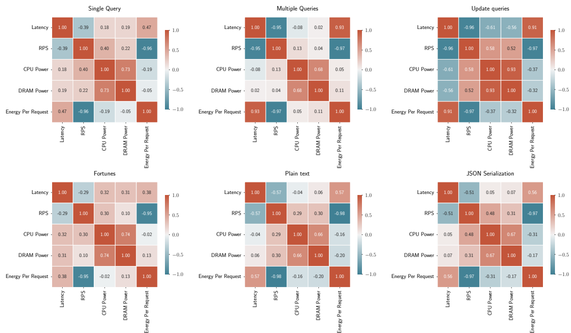
Figure 6.11: Spearman Rank Correlation between different metrics
