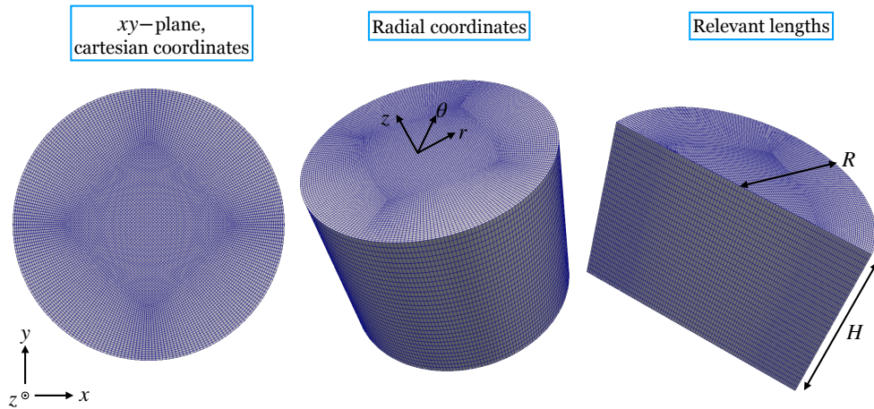
Figure 3.9 – A generic background mesh generated with the blockMesh utility, composed by an O-H butterfly topology. Left : the xy plane. The center square H block can be appreciated, along with the variation in resolution. Center : Radial coordinates. Right : Relevant lengths: the cylinder radius R and its height H .
