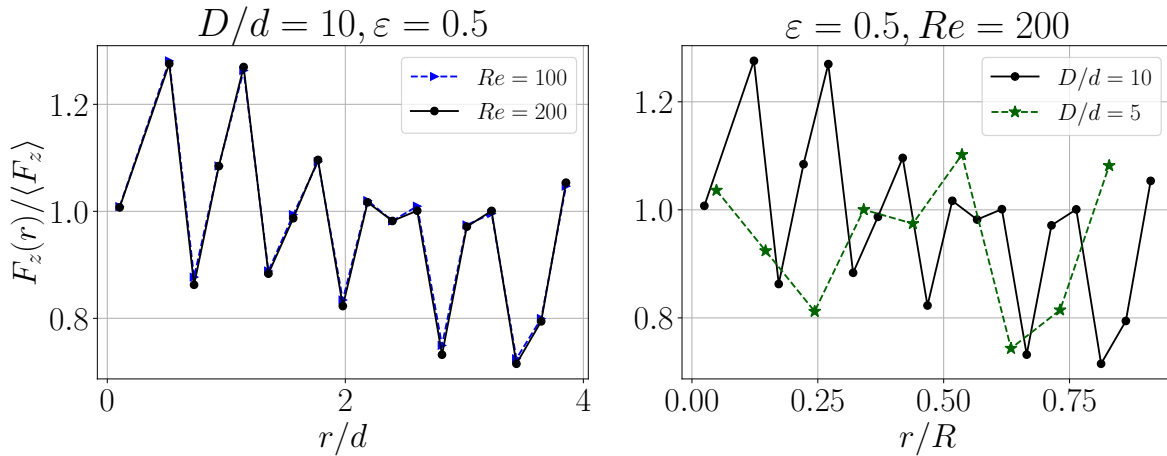
Figure 7.10 – Forces radial distribution for packed beds with D/d = 10 , \epsilon = 0.5 and two different Reynolds numbers Re = 100 and 200 (Left), and for two different cases with D/d = 5 and 10 with fixed porosity \epsilon = 0.5 and Re = 200 .
