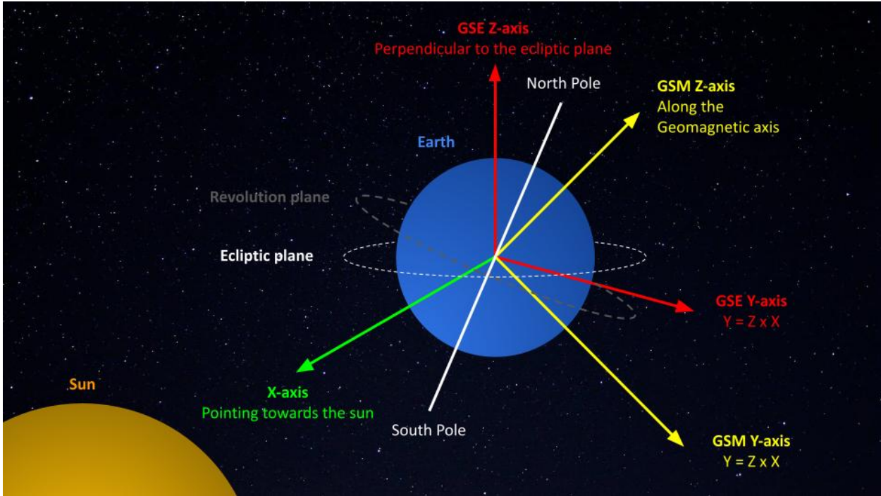
Figure A.1: Figure showing the difference between the GSE and GSM coordinate systems.
