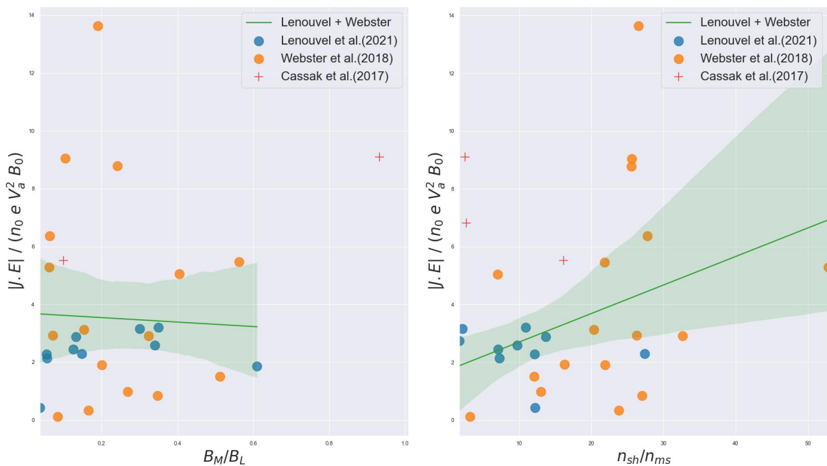
Figure 4.15: Scatterplots of the normalized absolute value of the energy conversion J.E as a function of the guide field B_M/B_L (left) and of the density asymmetry n_{sh}/n_{ms} (right)
