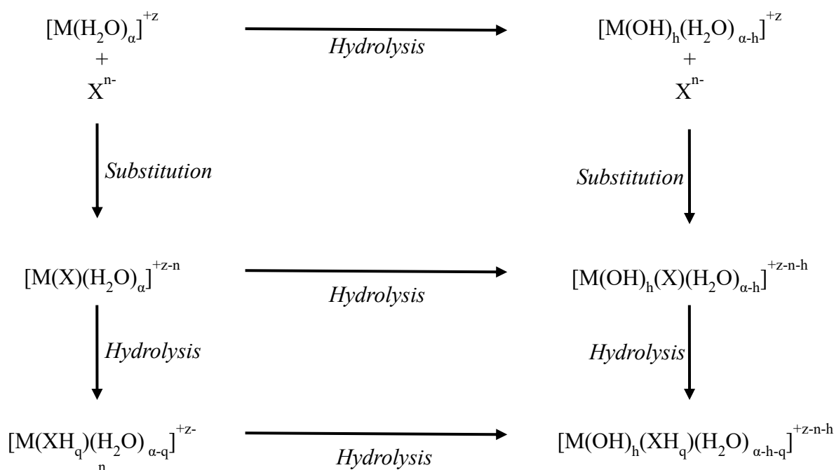
Figure 19: General complexes formed during hydrothermal synthesis with M the metal, X an anion with an n - charge, h the hydrolysis ratio of the cation, α the number of water molecules on the first hydration shell, z the charge of the cation, q the hydrolysis ratio of the anion. 24
