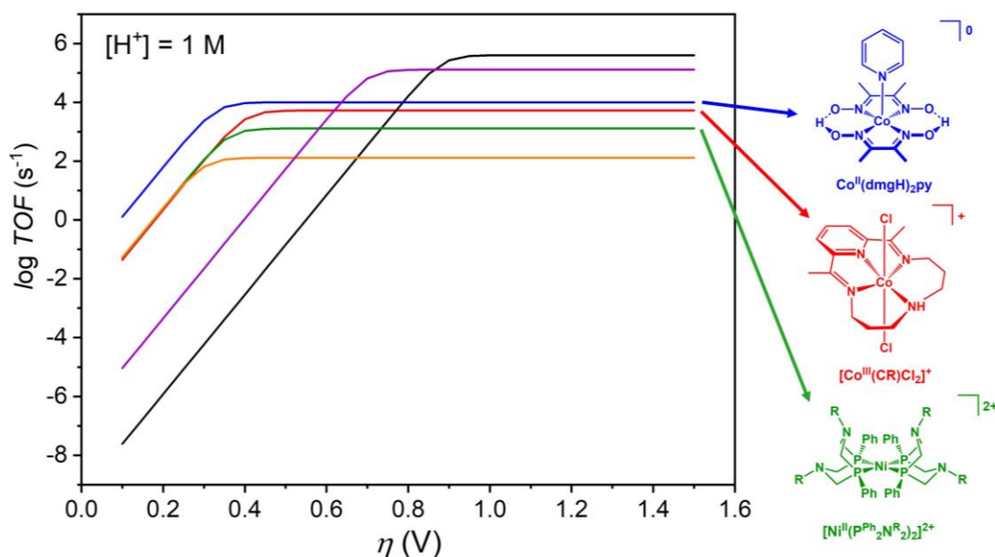
Figure 3.8: Catalytic Tafel plots of CAT1 (i.e. [\text{Co}^{\text{III}}(\text{CR})\text{Cl}_2]^+ ) in MeCN with pCNAH.BF 4 (red) against other competitor molecular catalysts: Iron tetraphenylporphyrin, \text{Fe}^{\text{II}}\text{TPP} in DMF with \text{Et}_3\text{NH}^+ (black), pyridine-cobaloxime, \text{Co}^{\text{II}}(\text{dmgH})_2\text{py} in DMF with \text{Et}_3\text{NH}^+ (blue), phenylphosphine DuBois catalyst with phosphonate ester groups, [\text{Ni}^{\text{II}}(\text{P}^{\text{Ph}}_2\text{NR}_2)_2]^{2+} , \text{R} = p\text{-C}_6\text{H}_4\text{-CH}_2\text{P}(\text{O})(\text{OEt})_2 in MeCN with DMFH + (green), a cobalt bithiosemicarbazone in DMF with \text{Et}_3\text{NH}^+ (orange), and a cobalt polypyridine complex, [\text{Co}^{\text{II}}(\text{bapbpy})\text{Cl}]^+ in DMF with \text{Et}_3\text{NH}^+ (purple). \eta = applied overpotential for the HER. Reproduced from Paper I with permission from the Royal Society of Chemistry. Note the position of the red line for CAT1 with TOF max between the green (DuBois) and blue (cobaloxime).
