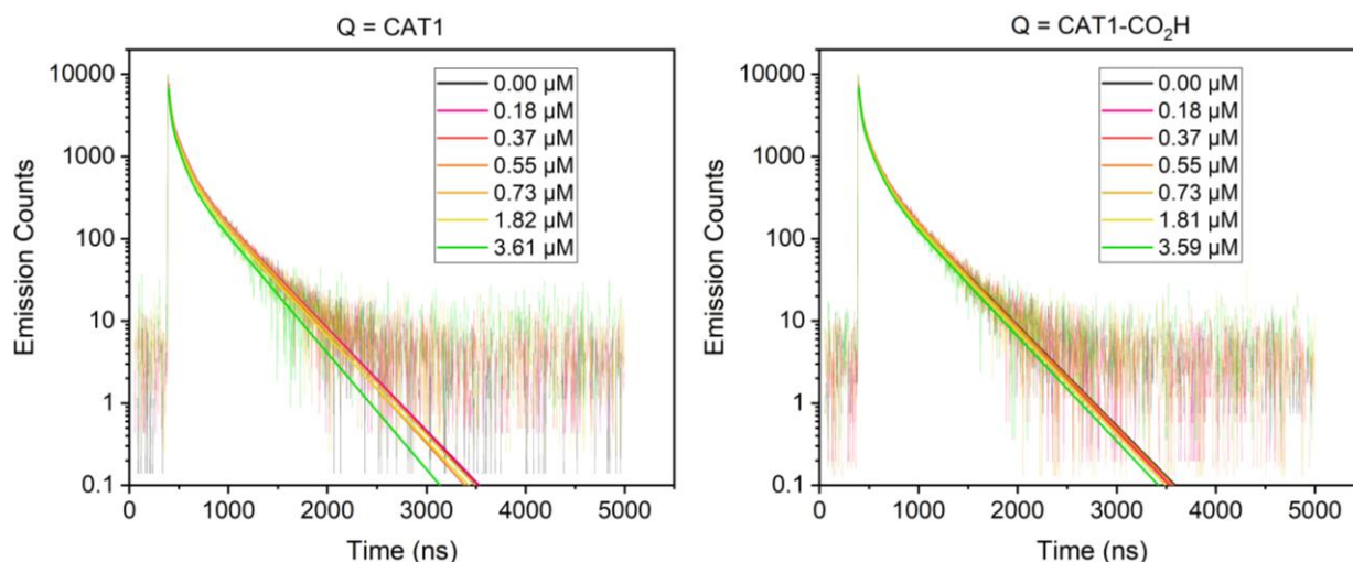
Figure 5.5: Example TCSPC traces and rough triexponential fits for the same samples as in Figure 5.4 : A CIS QD sample diluted to have an absorbance of 0.07 at 405 nm (estimated [QD]: approximately 1 \mu\text{M} ) with increasing concentration of either CAT1 ( Left ) or CAT1-CO 2 H ( Right ). PL excitation wavelength for TCSPC: 470 nm. Cuvette pathlength: 1 cm. Solvent: deionised water.
