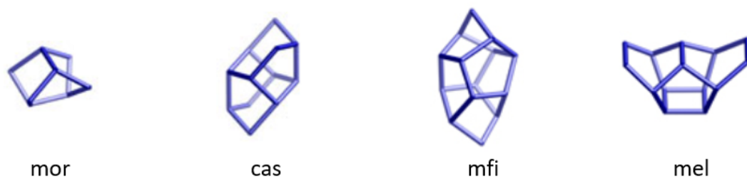
Figure 1.7: Composite Building Units CBU involved in the formation of the MFI zeolite structure. The arrangement of these units allows building channels [42].
